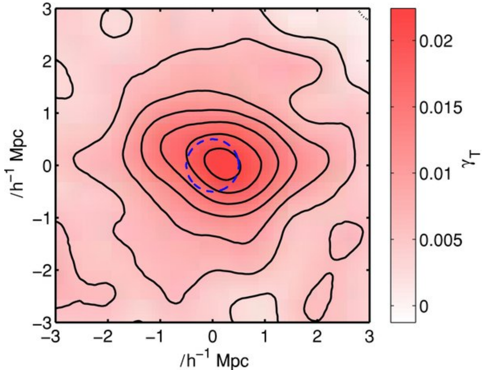
Figure 2. from A Detection of Dark Matter Halo Ellipticity using Galaxy Cluster Lensing in the SDSS EVANS & BRIDLE 2009 ApJ 695 1446 doi:10.1088/0004-637X/695/2/1446 https://dx.doi.org/10.1088/0004-637X/695/2/1446 © 2009. The American Astronomical Society. All rights reserved.
