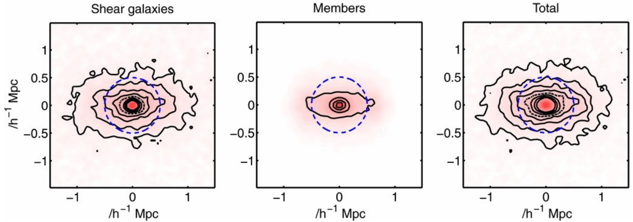
Figure 1. from A Detection of Dark Matter Halo Ellipticity using Galaxy Cluster Lensing in the SDSS EVANS & BRIDLE 2009 ApJ 695 1446 doi:10.1088/0004-637X/695/2/1446 https://dx.doi.org/10.1088/0004-637X/695/2/1446 © 2009. The American Astronomical Society. All rights reserved.
