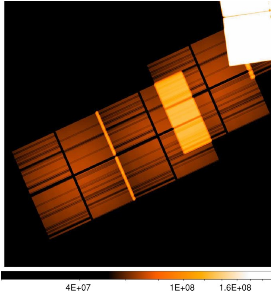
Figure 8. from A Chandra Study of the Rosette Star-Forming Complex. II. Clusters in the Rosette Molecular Cloud WANG ET AL. 2009 ApJ 696 47 doi:10.1088/0004-637X/696/1/47 https://dx.doi.org/10.1088/0004-637X/696/1/47 © 2009. The American Astronomical Society. All rights reserved.
