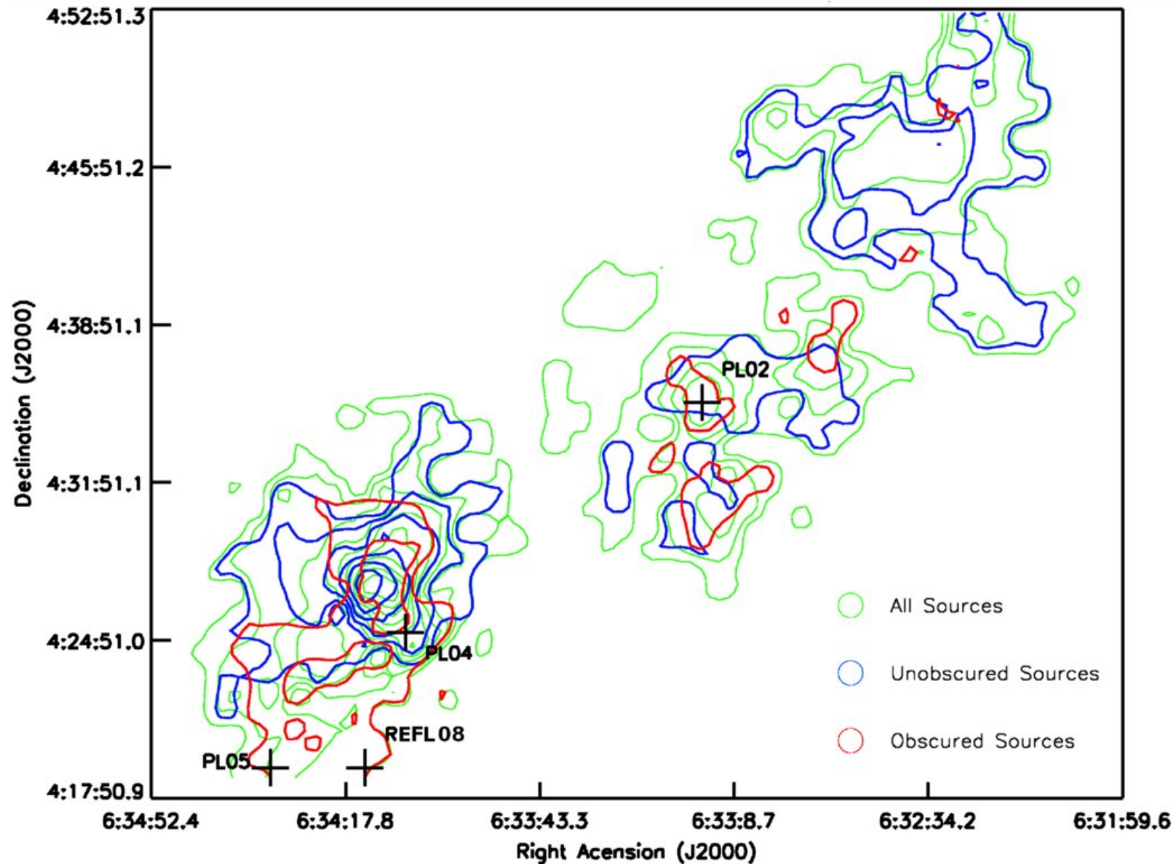
Figure 7. from A Chandra Study of the Rosette Star-Forming Complex. II. Clusters in the Rosette Molecular Cloud WANG ET AL. 2009 ApJ 696 47 doi:10.1088/0004-637X/696/1/47 https://dx.doi.org/10.1088/0004-637X/696/1/47 © 2009. The American Astronomical Society. All rights reserved.
