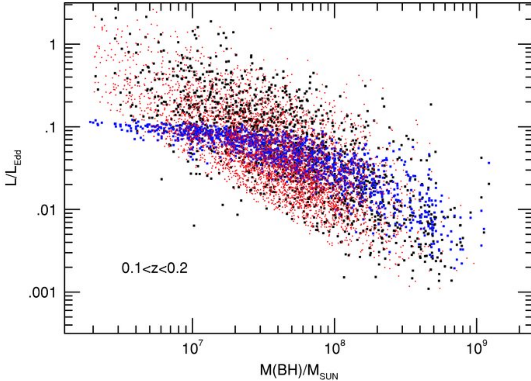
Figure 4. from Radiation Pressure Force and Black Hole Mass Determination in Low-Redshift Type-I and Type-II Active Galactic Nuclei NETZER 2009 ApJ 695 793 doi:10.1088/0004-637X/695/1/793 https://dx.doi.org/10.1088/0004-637X/695/1/793 © 2009. The American Astronomical Society. All rights reserved.
