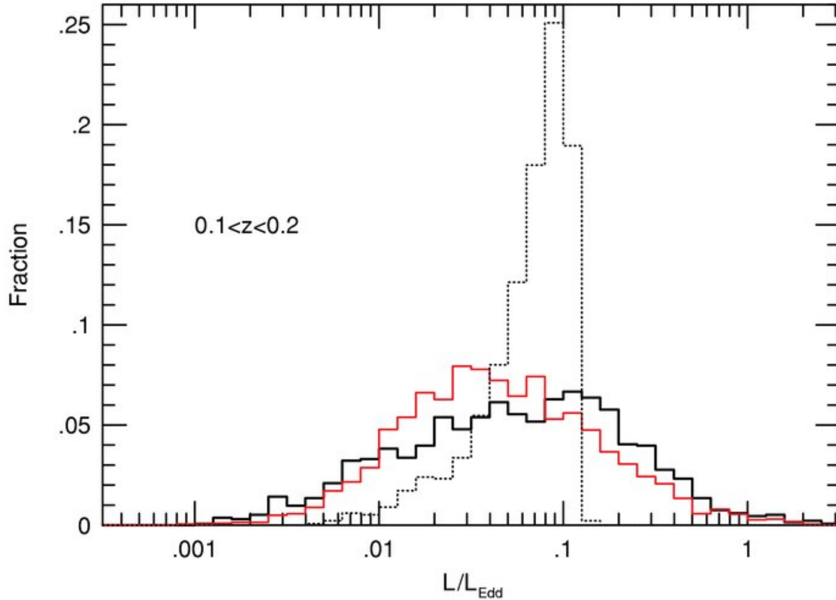
Figure 3. from Radiation Pressure Force and Black Hole Mass Determination in Low-Redshift Type-I and Type-II Active Galactic Nuclei NETZER 2009 ApJ 695 793 doi:10.1088/0004-637X/695/1/793 https://dx.doi.org/10.1088/0004-637X/695/1/793 © 2009. The American Astronomical Society. All rights reserved.
