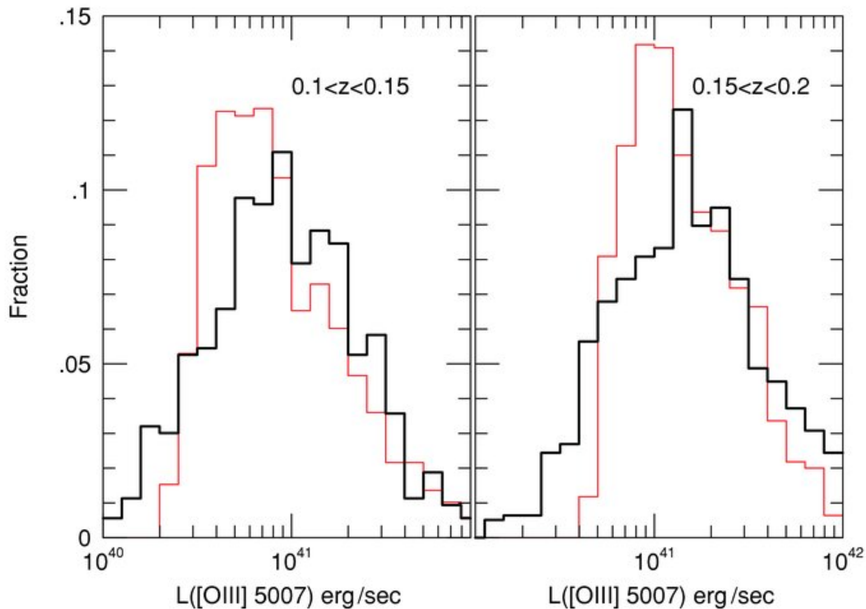
Figure 1. from Radiation Pressure Force and Black Hole Mass Determination in Low-Redshift Type-I and Type-II Active Galactic Nuclei NETZER 2009 ApJ 695 793 doi:10.1088/0004-637X/695/1/793 https://dx.doi.org/10.1088/0004-637X/695/1/793 © 2009. The American Astronomical Society. All rights reserved.
