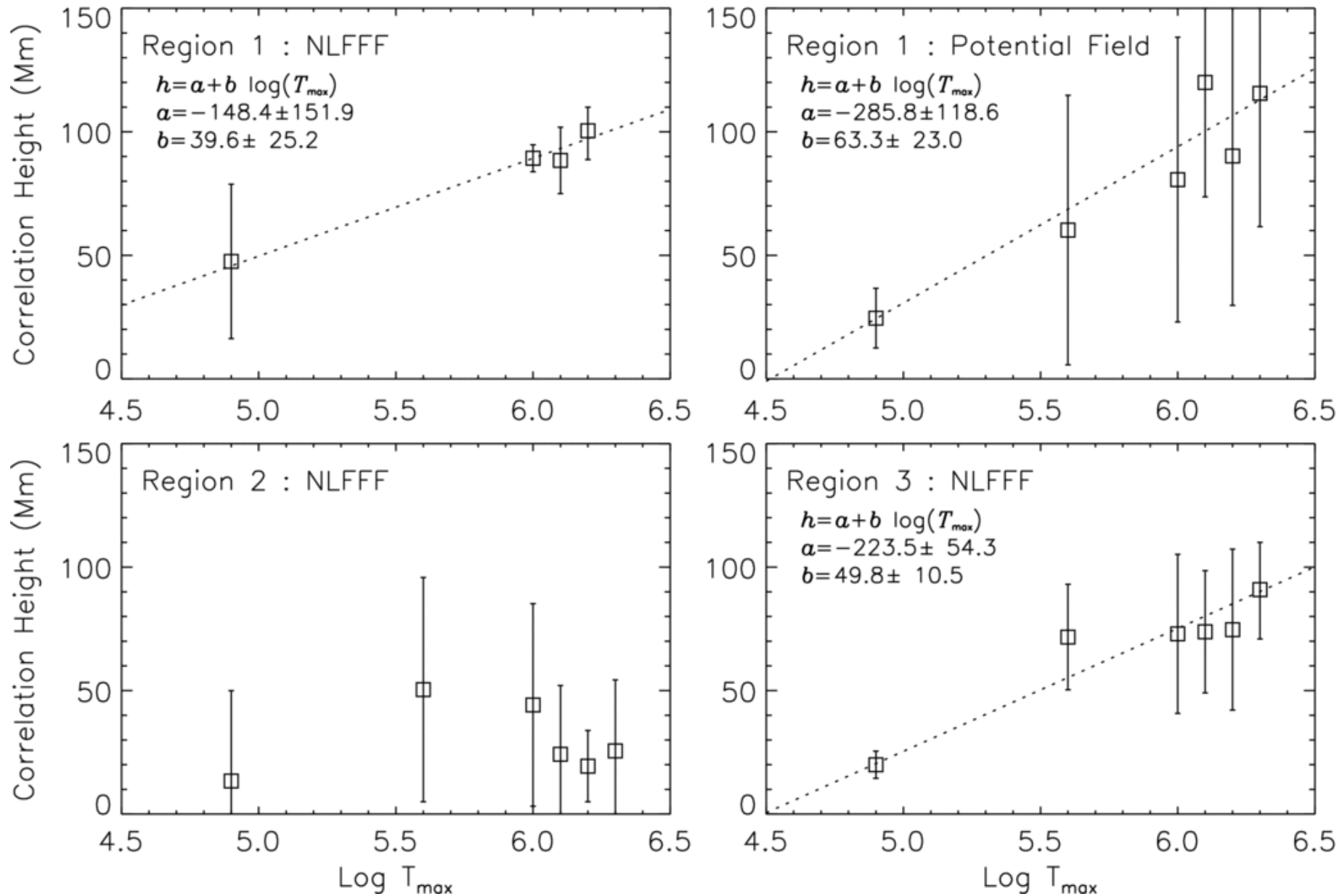
Figure 5. from Formation Heights of Extreme Ultraviolet Lines in an Active Region Derived by Correlation of Doppler Velocity and Magnetic Field GUO ET AL. 2009 ApJ 696 1526 doi:10.1088/0004-637X/696/2/1526 https://dx.doi.org/10.1088/0004-637X/696/2/1526 © 2009. The American Astronomical Society. All rights reserved.
