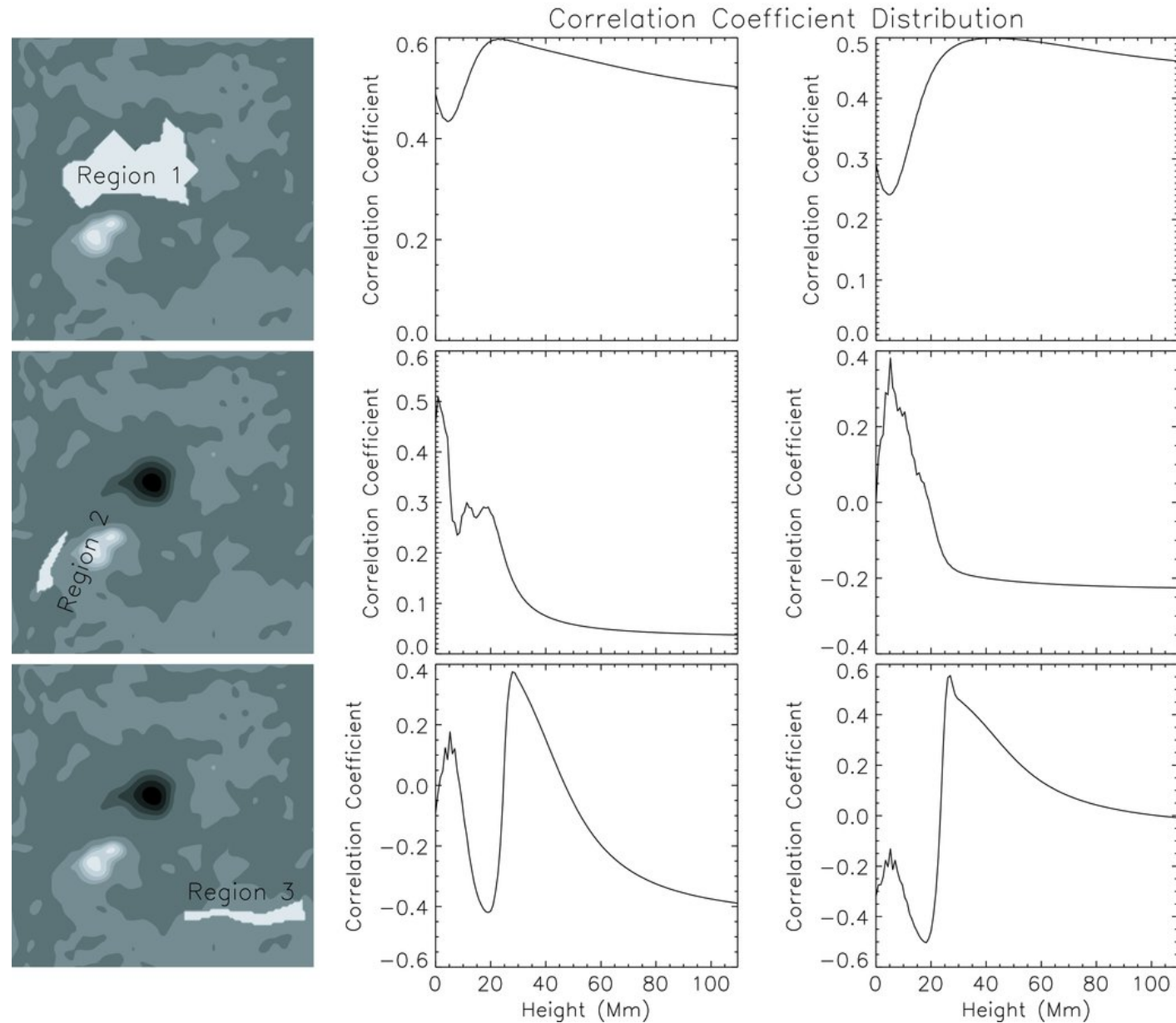
Figure 4. from Formation Heights of Extreme Ultraviolet Lines in an Active Region Derived by Correlation of Doppler Velocity and Magnetic Field GUO ET AL. 2009 ApJ 696 1526 doi:10.1088/0004-637X/696/2/1526 https://dx.doi.org/10.1088/0004-637X/696/2/1526 © 2009. The American Astronomical Society. All rights reserved.
