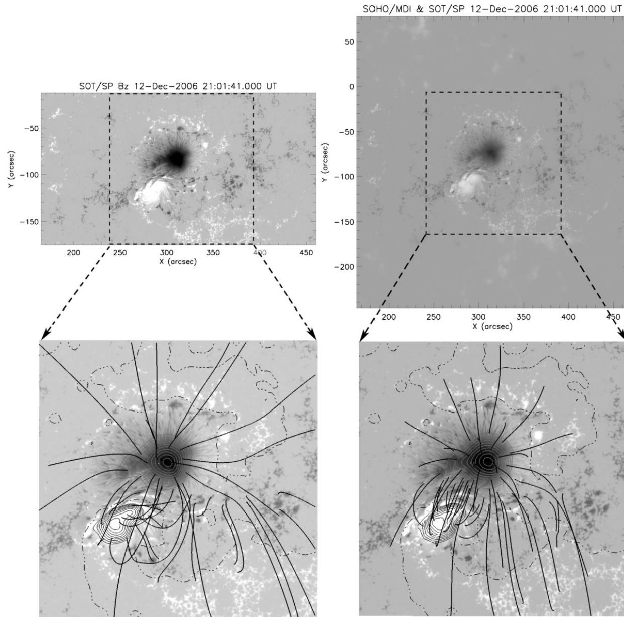
Figure 2. from Formation Heights of Extreme Ultraviolet Lines in an Active Region Derived by Correlation of Doppler Velocity and Magnetic Field GUO ET AL. 2009 ApJ 696 1526 doi:10.1088/0004-637X/696/2/1526 https://dx.doi.org/10.1088/0004-637X/696/2/1526 © 2009. The American Astronomical Society. All rights reserved.
