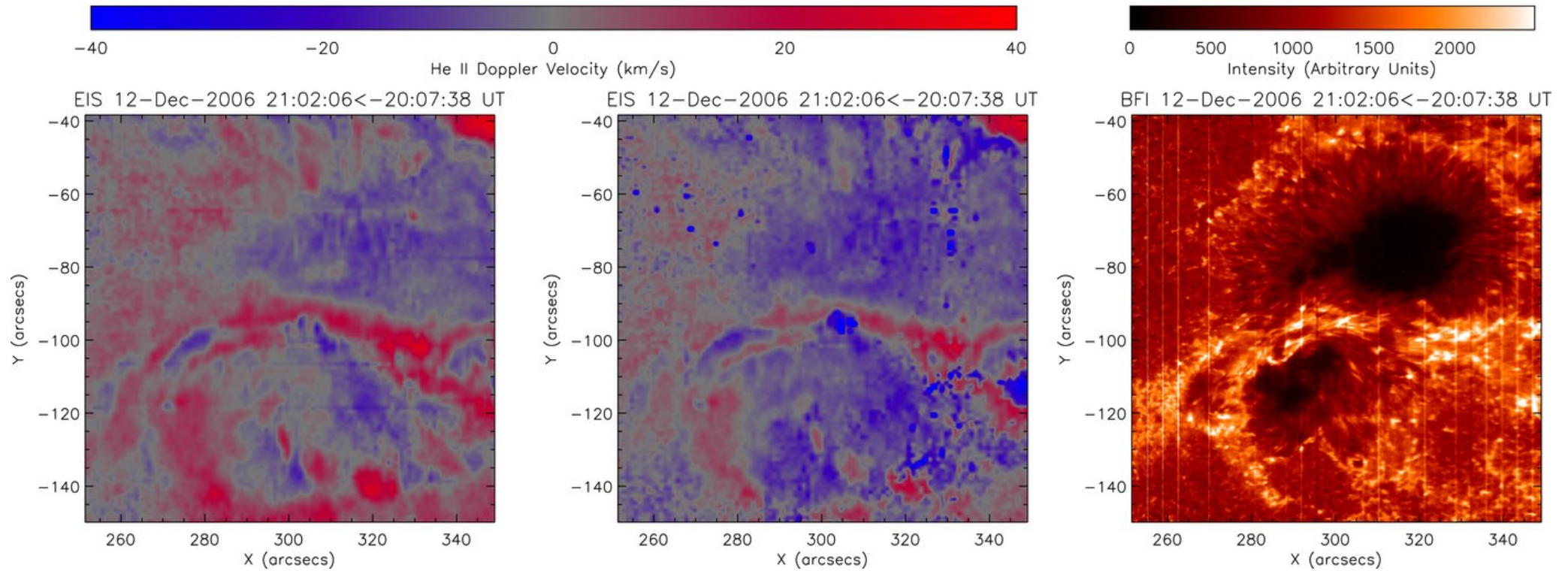
Figure 1. from Formation Heights of Extreme Ultraviolet Lines in an Active Region Derived by Correlation of Doppler Velocity and Magnetic Field GUO ET AL. 2009 ApJ 696 1526 doi:10.1088/0004-637X/696/2/1526 https://dx.doi.org/10.1088/0004-637X/696/2/1526 © 2009. The American Astronomical Society. All rights reserved.
