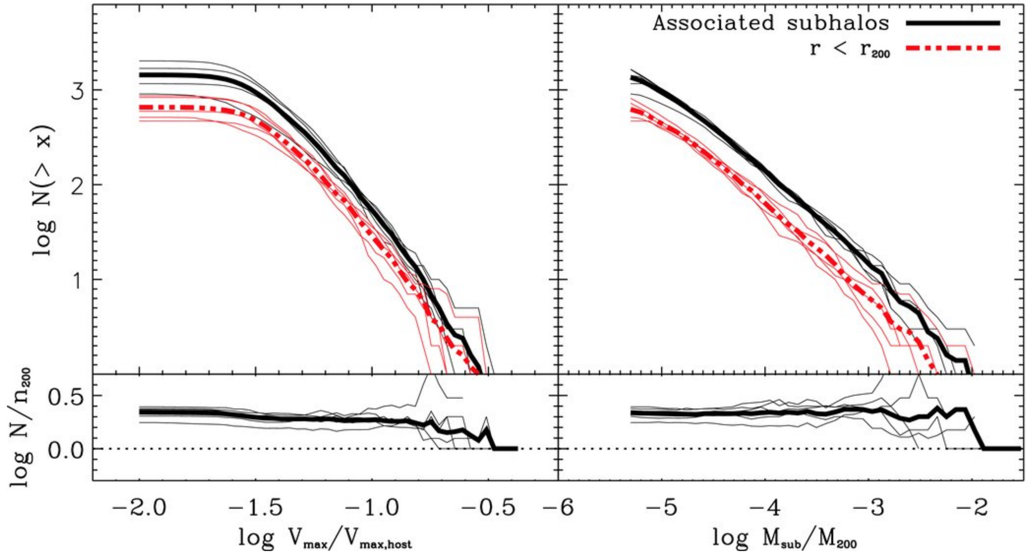
Figure 8. from The Unorthodox Orbits of Substructure Halos LUDLOW ET AL. 2009 ApJ 692 931 doi:10.1088/0004-637X/692/1/931 https://dx.doi.org/10.1088/0004-637X/692/1/931 © 2009. The American Astronomical Society. All rights reserved.
