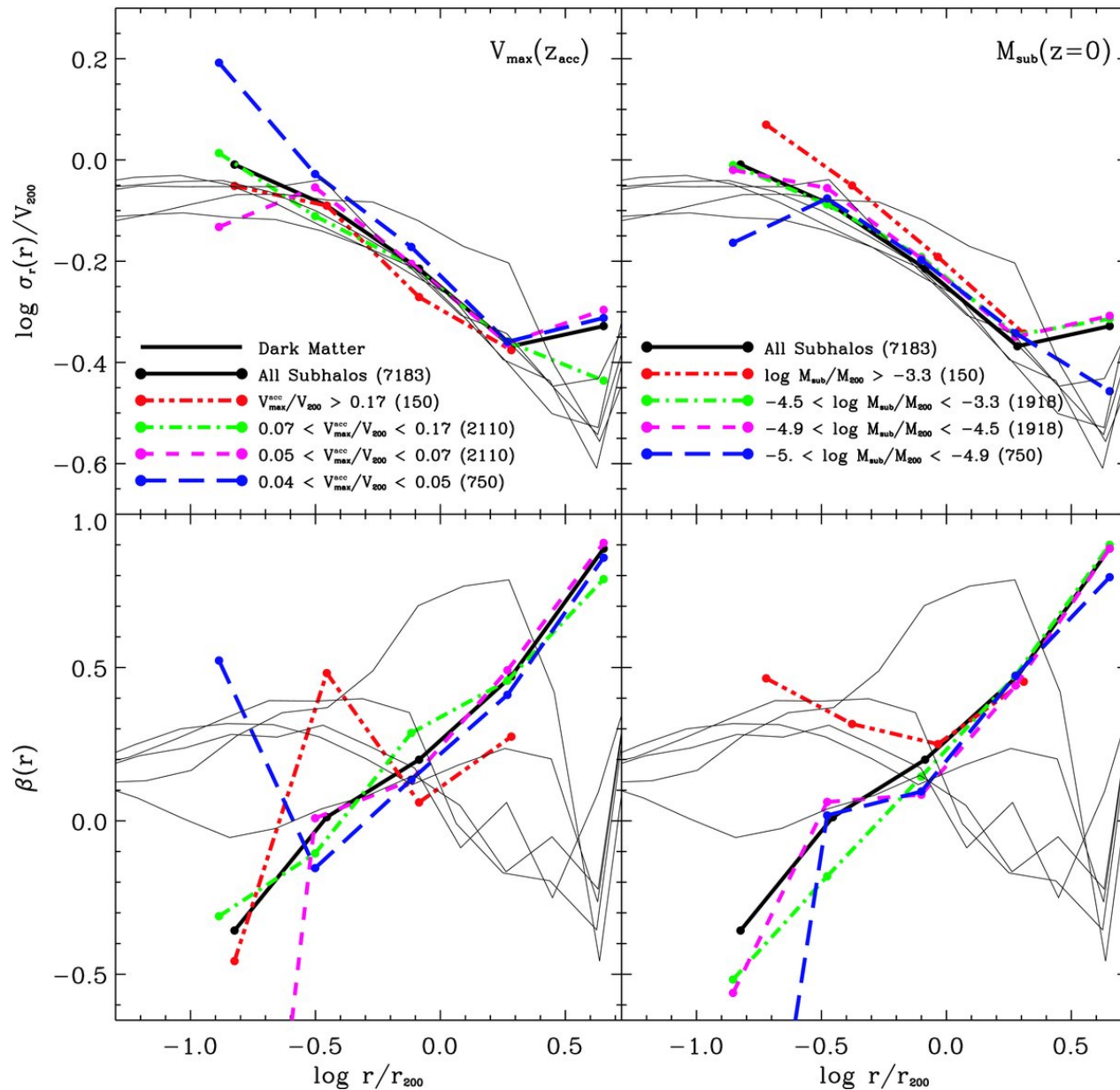
Figure 7. from The Unorthodox Orbits of Substructure Halos LUDLOW ET AL. 2009 ApJ 692 931 doi:10.1088/0004-637X/692/1/931 https://dx.doi.org/10.1088/0004-637X/692/1/931 © 2009. The American Astronomical Society. All rights reserved.
