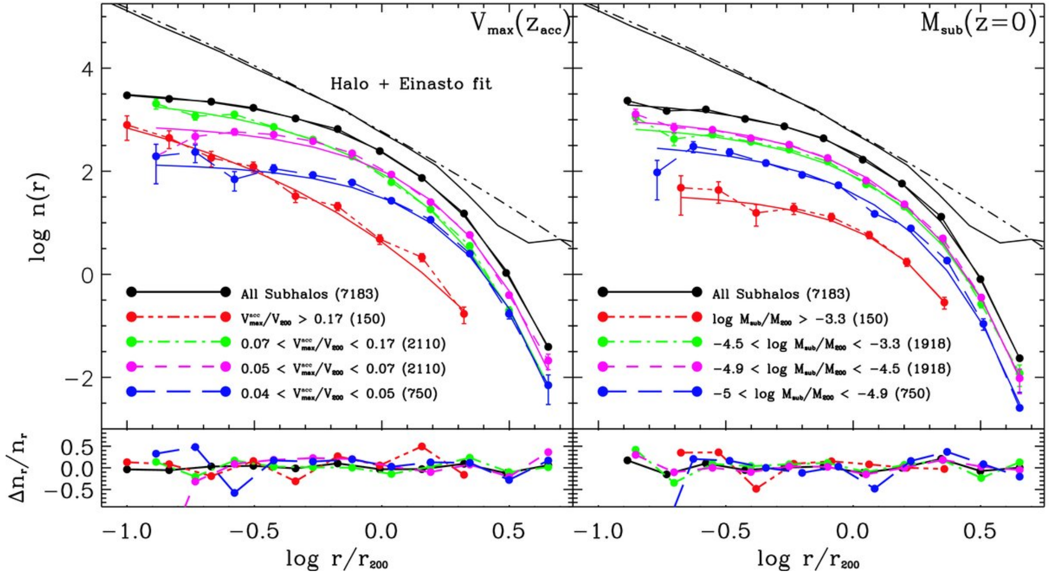
Figure 6. from The Unorthodox Orbits of Substructure Halos LUDLOW ET AL. 2009 ApJ 692 931 doi:10.1088/0004-637X/692/1/931 https://dx.doi.org/10.1088/0004-637X/692/1/931 © 2009. The American Astronomical Society. All rights reserved.
