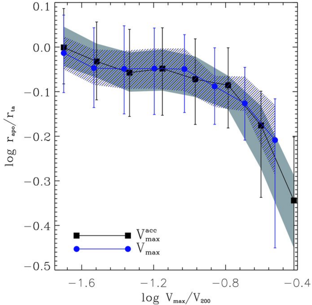
Figure 5. from The Unorthodox Orbits of Substructure Halos LUDLOW ET AL. 2009 ApJ 692 931 doi:10.1088/0004-637X/692/1/931 https://dx.doi.org/10.1088/0004-637X/692/1/931 © 2009. The American Astronomical Society. All rights reserved.
