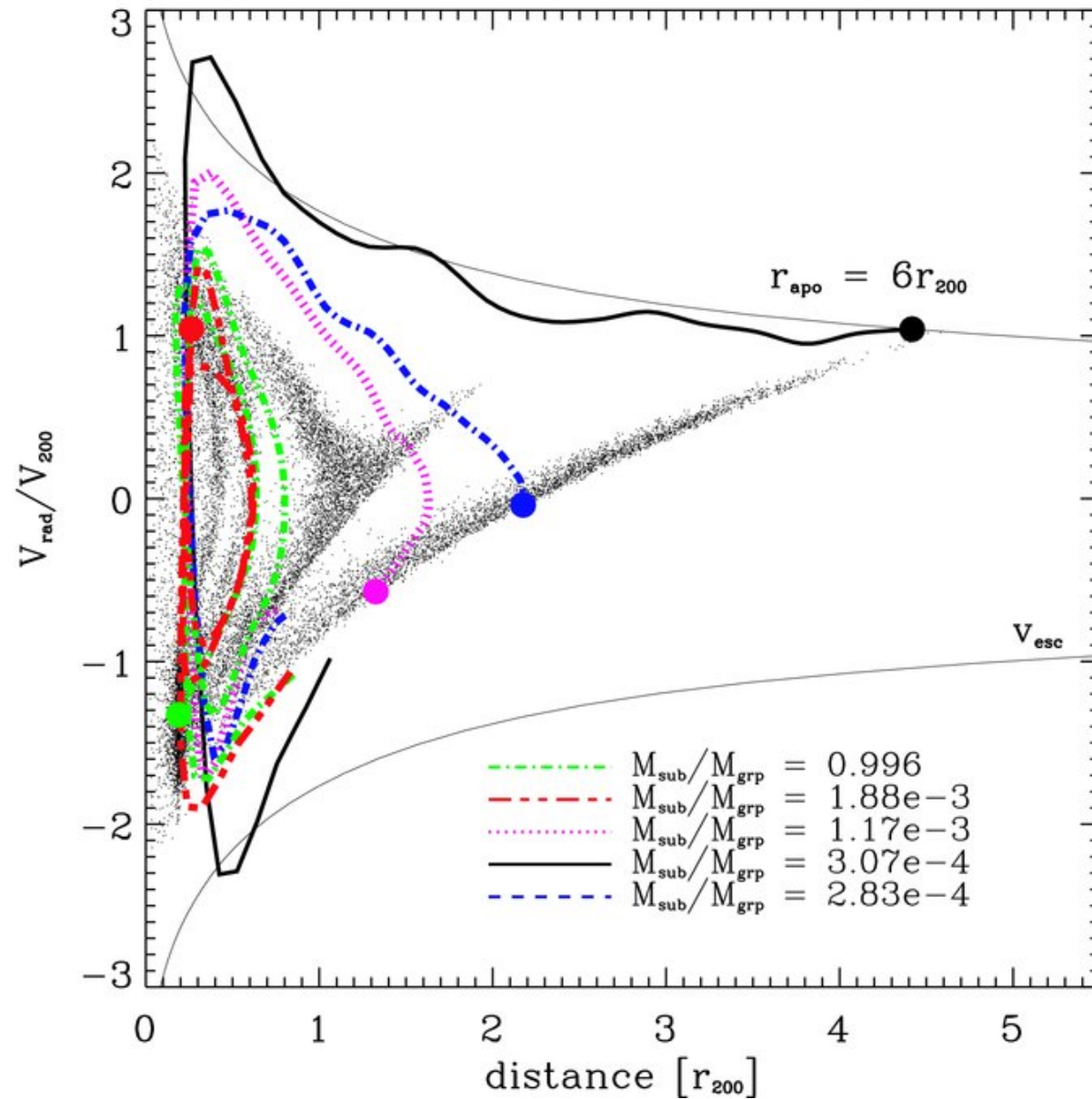
Figure 4. from The Unorthodox Orbits of Substructure Halos LUDLOW ET AL. 2009 ApJ 692 931 doi:10.1088/0004-637X/692/1/931 https://dx.doi.org/10.1088/0004-637X/692/1/931 © 2009. The American Astronomical Society. All rights reserved.
