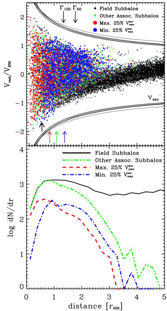
Figure 1. from The Unorthodox Orbits of Substructure Halos LUDLOW ET AL. 2009 ApJ 692 931 doi:10.1088/0004-637X/692/1/931 https://dx.doi.org/10.1088/0004-637X/692/1/931 © 2009. The American Astronomical Society. All rights reserved.
