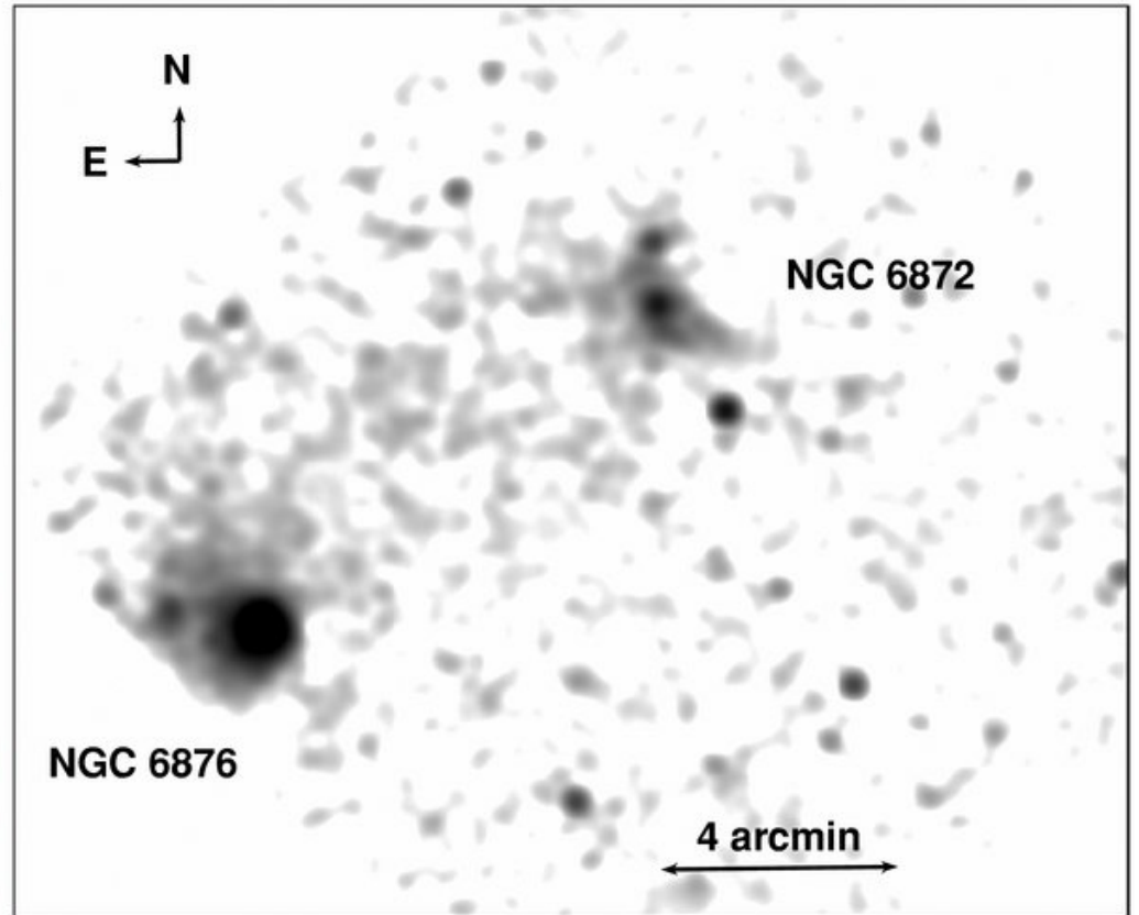
Figure 7. from A MULTIWAVELENGTH VIEW OF STAR FORMATION IN INTERACTING GALAXIES IN THE PAVO GROUP MACHACEK ET AL. 2009 ApJ 691 1921 doi:10.1088/0004-637X/691/2/1921 https://dx.doi.org/10.1088/0004-637X/691/2/1921 © 2009. The American Astronomical Society. All rights reserved.
