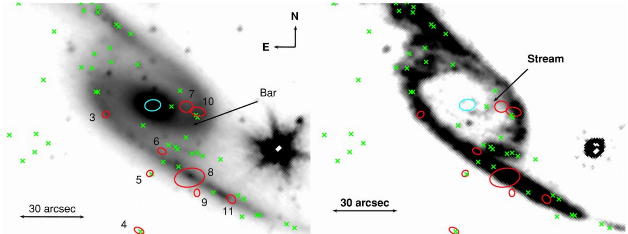
Figure 6. from A MULTIWAVELENGTH VIEW OF STAR FORMATION IN INTERACTING GALAXIES IN THE PAVO GROUP MACHACEK ET AL. 2009 ApJ 691 1921 doi:10.1088/0004-637X/691/2/1921 https://dx.doi.org/10.1088/0004-637X/691/2/1921 © 2009. The American Astronomical Society. All rights reserved.
