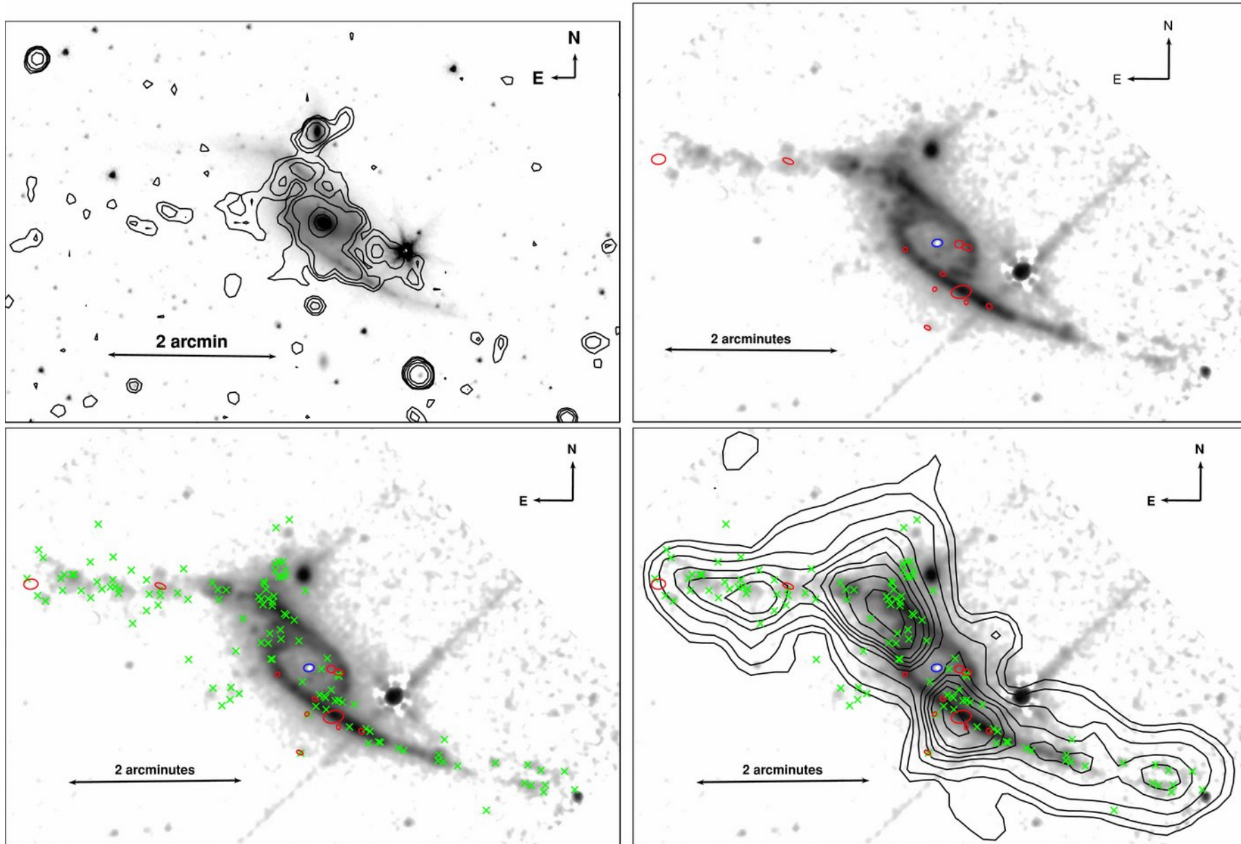
Figure 5. from A MULTIWAVELENGTH VIEW OF STAR FORMATION IN INTERACTING GALAXIES IN THE PAVO GROUP MACHACEK ET AL. 2009 ApJ 691 1921 doi:10.1088/0004-637X/691/2/1921 https://dx.doi.org/10.1088/0004-637X/691/2/1921 © 2009. The American Astronomical Society. All rights reserved.
