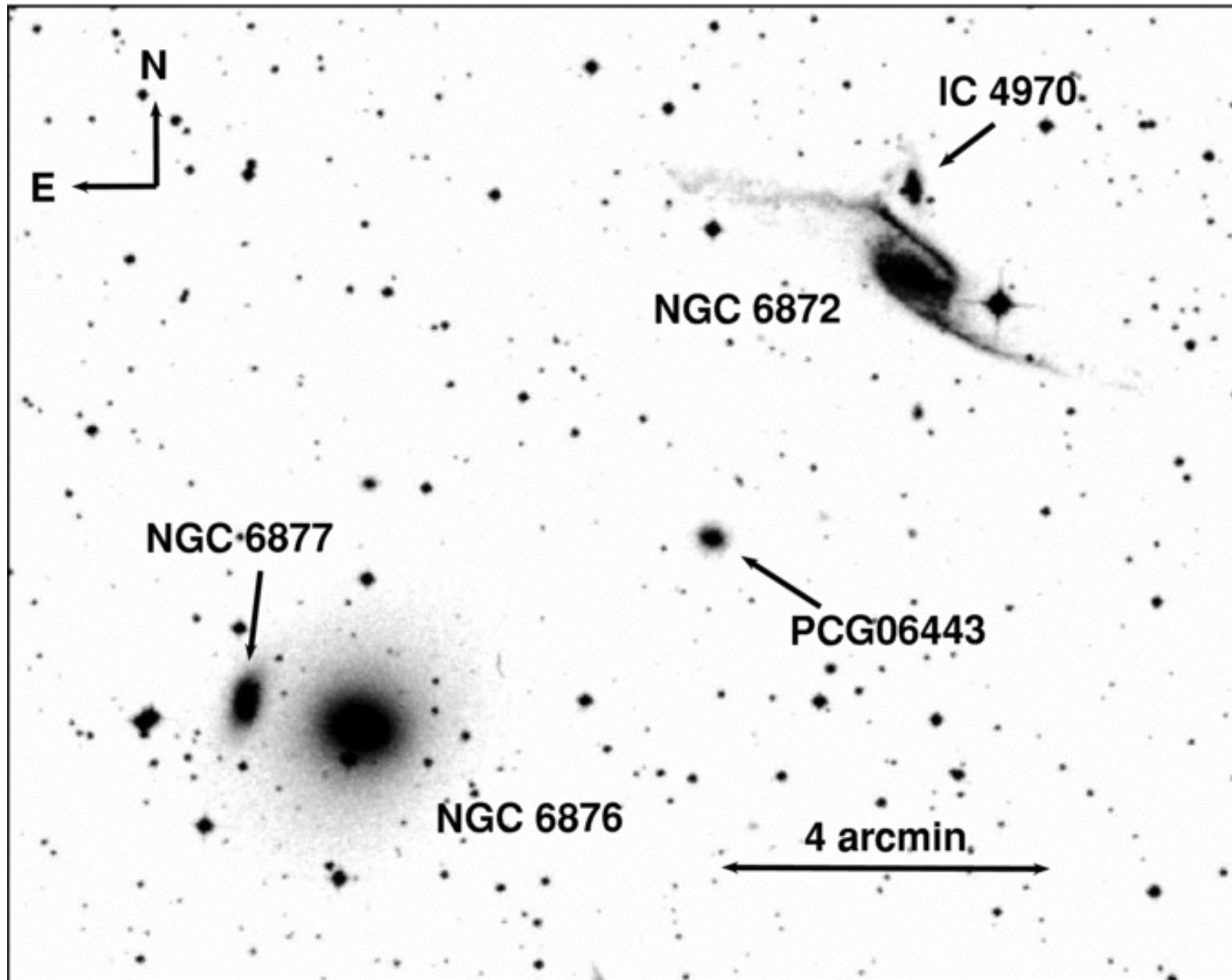
Figure 1. from A MULTIWAVELENGTH VIEW OF STAR FORMATION IN INTERACTING GALAXIES IN THE PAVO GROUP MACHACEK ET AL. 2009 ApJ 691 1921 doi:10.1088/0004-637X/691/2/1921 https://dx.doi.org/10.1088/0004-637X/691/2/1921 © 2009. The American Astronomical Society. All rights reserved.
