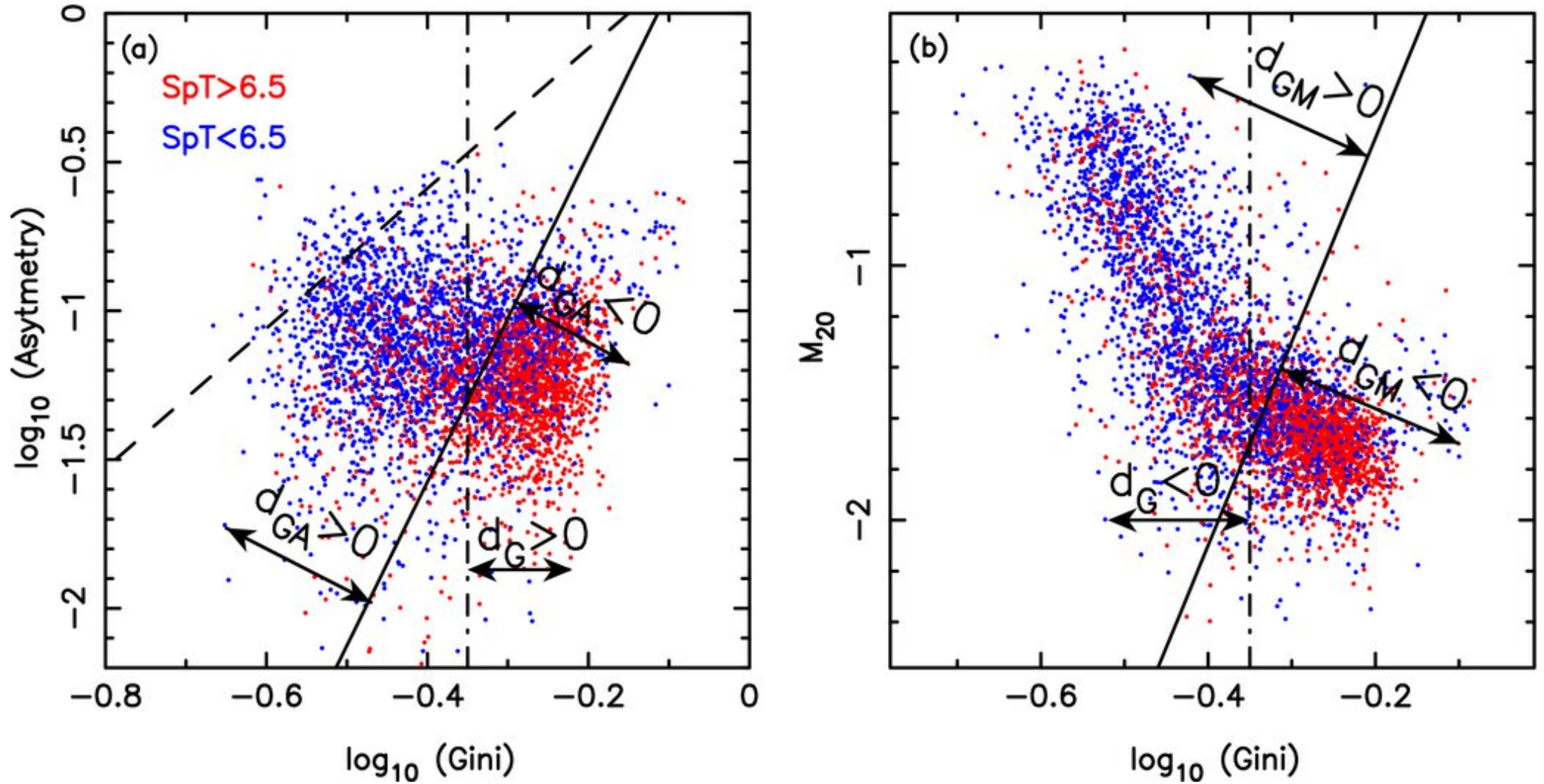
Figure 7. from Classification of Extremely Red Objects in the Cosmos Field KONG ET AL. 2009 ApJ 702 1458 doi:10.1088/0004-637X/702/2/1458 https://dx.doi.org/10.1088/0004-637X/702/2/1458 © 2009. The American Astronomical Society. All rights reserved.
