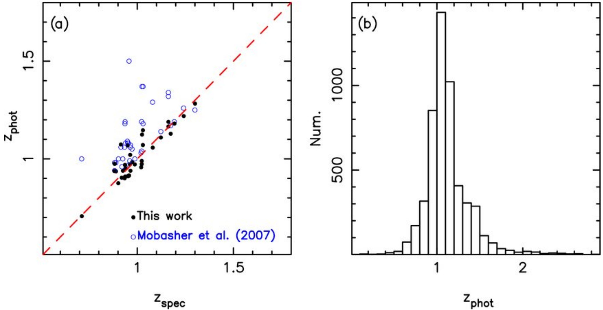
Figure 3. from Classification of Extremely Red Objects in the Cosmos Field KONG ET AL. 2009 ApJ 702 1458 doi:10.1088/0004-637X/702/2/1458 https://dx.doi.org/10.1088/0004-637X/702/2/1458 © 2009. The American Astronomical Society. All rights reserved.
