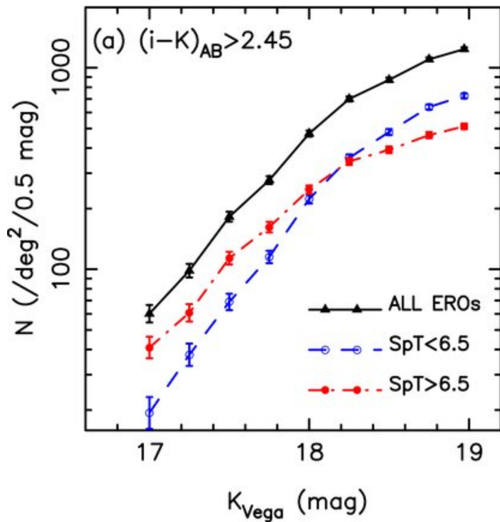
Figure 10. from Classification of Extremely Red Objects in the Cosmos Field KONG ET AL. 2009 ApJ 702 1458 doi:10.1088/0004-637X/702/2/1458 https://dx.doi.org/10.1088/0004-637X/702/2/1458 © 2009. The American Astronomical Society. All rights reserved.
