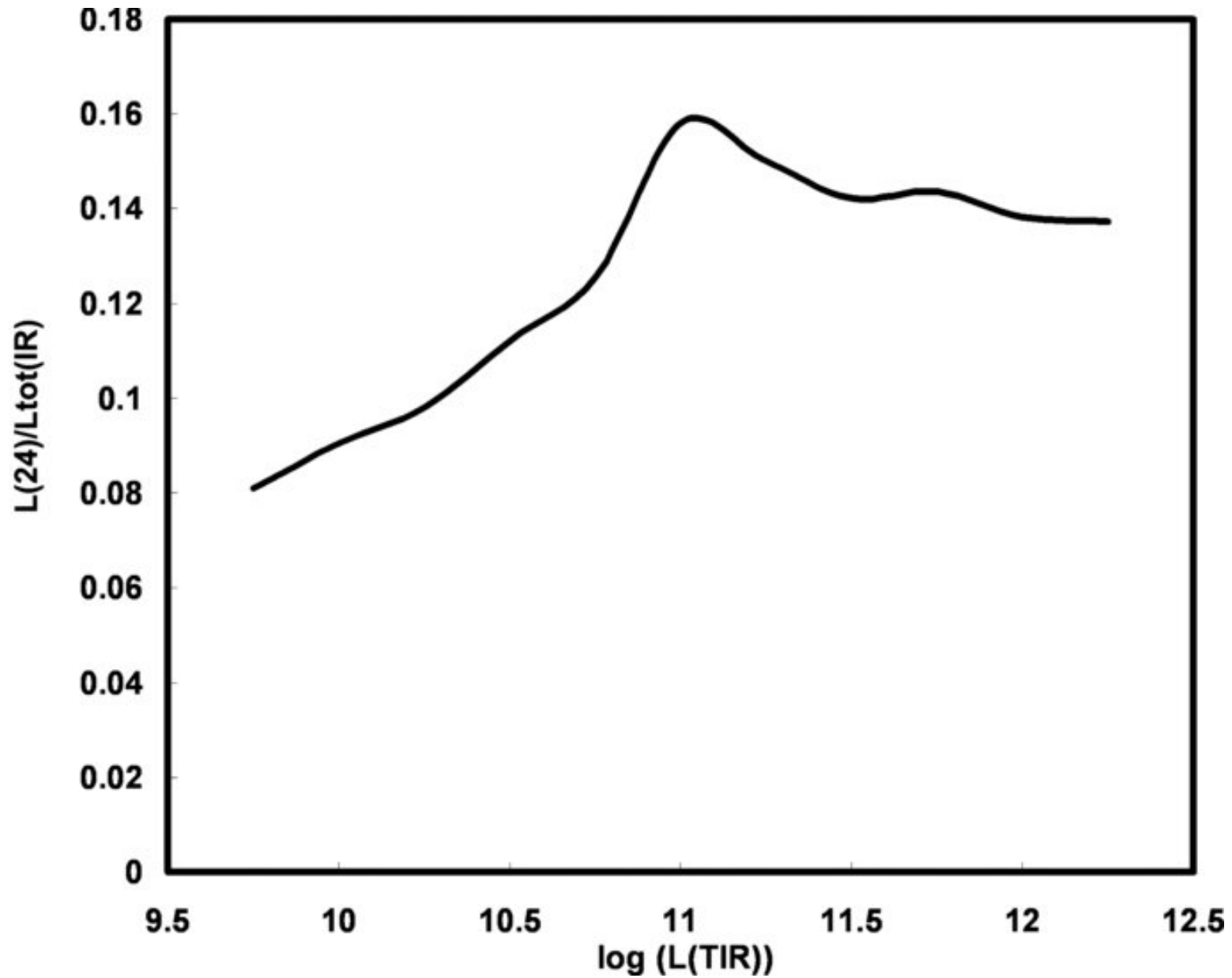
Figure 8. from Determining Star Formation Rates for Infrared Galaxies RIEKE ET AL. 2009 ApJ 692 556 doi:10.1088/0004-637X/692/1/556 https://dx.doi.org/10.1088/0004-637X/692/1/556 © 2009. The American Astronomical Society. All rights reserved.
