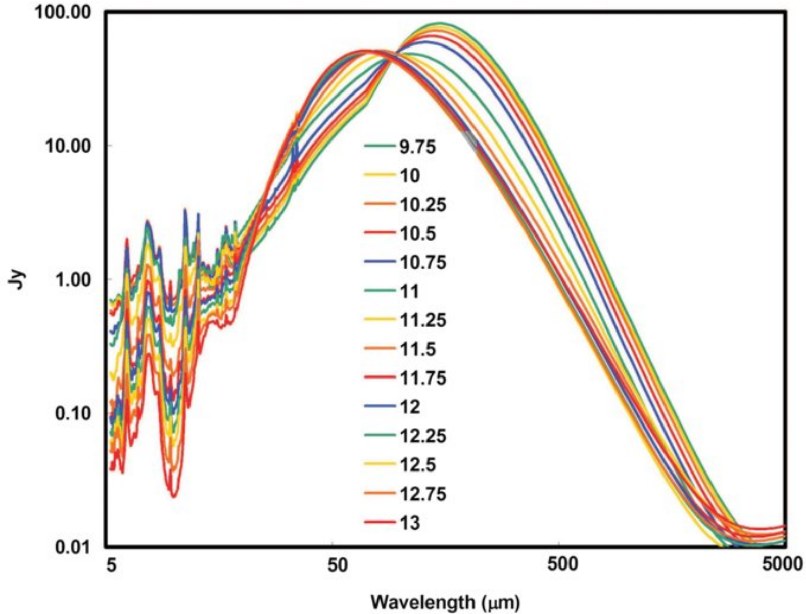
Figure 6. from Determining Star Formation Rates for Infrared Galaxies RIEKE ET AL. 2009 ApJ 692 556 doi:10.1088/0004-637X/692/1/556 https://dx.doi.org/10.1088/0004-637X/692/1/556 © 2009. The American Astronomical Society. All rights reserved.
