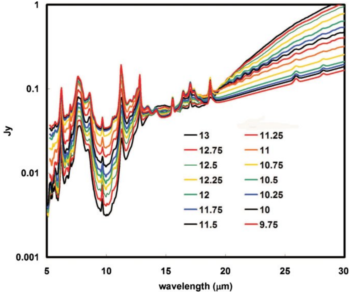
Figure 5. from Determining Star Formation Rates for Infrared Galaxies RIEKE ET AL. 2009 ApJ 692 556 doi:10.1088/0004-637X/692/1/556 https://dx.doi.org/10.1088/0004-637X/692/1/556 © 2009. The American Astronomical Society. All rights reserved.
