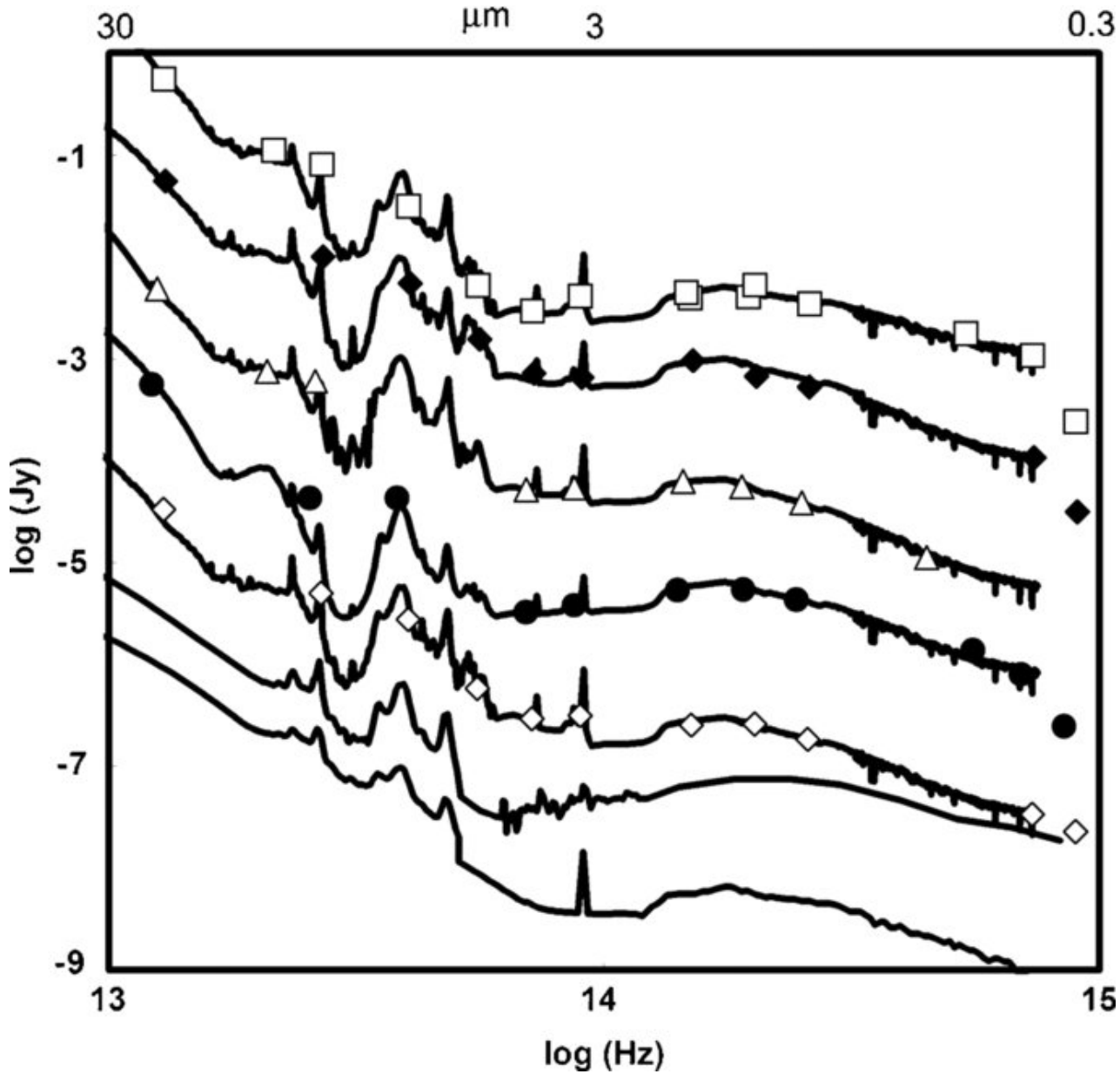
Figure 4. from Determining Star Formation Rates for Infrared Galaxies RIEKE ET AL. 2009 ApJ 692 556 doi:10.1088/0004-637X/692/1/556 https://dx.doi.org/10.1088/0004-637X/692/1/556 © 2009. The American Astronomical Society. All rights reserved.
