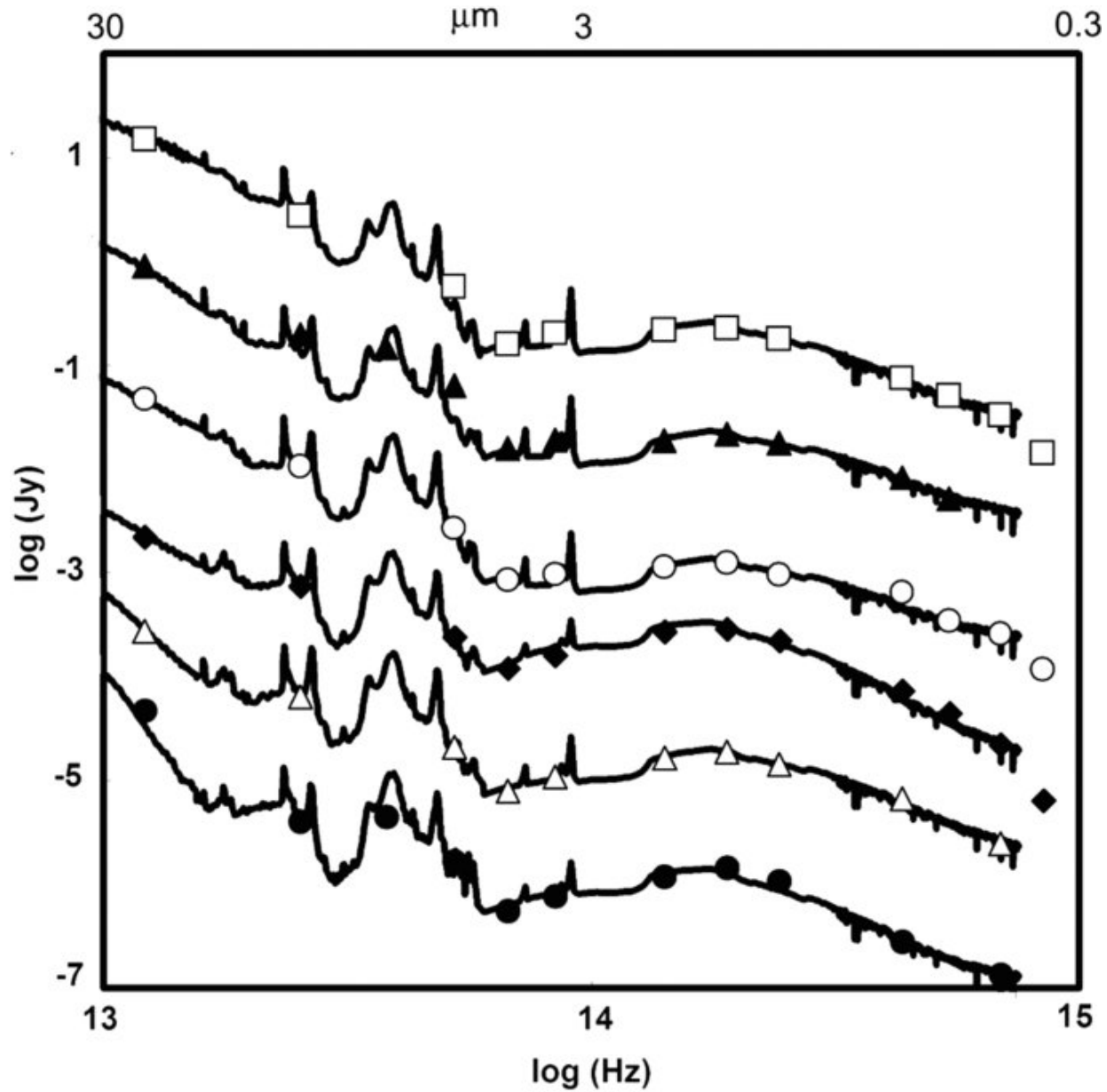
Figure 2. from Determining Star Formation Rates for Infrared Galaxies RIEKE ET AL. 2009 ApJ 692 556 doi:10.1088/0004-637X/692/1/556 https://dx.doi.org/10.1088/0004-637X/692/1/556 © 2009. The American Astronomical Society. All rights reserved.
