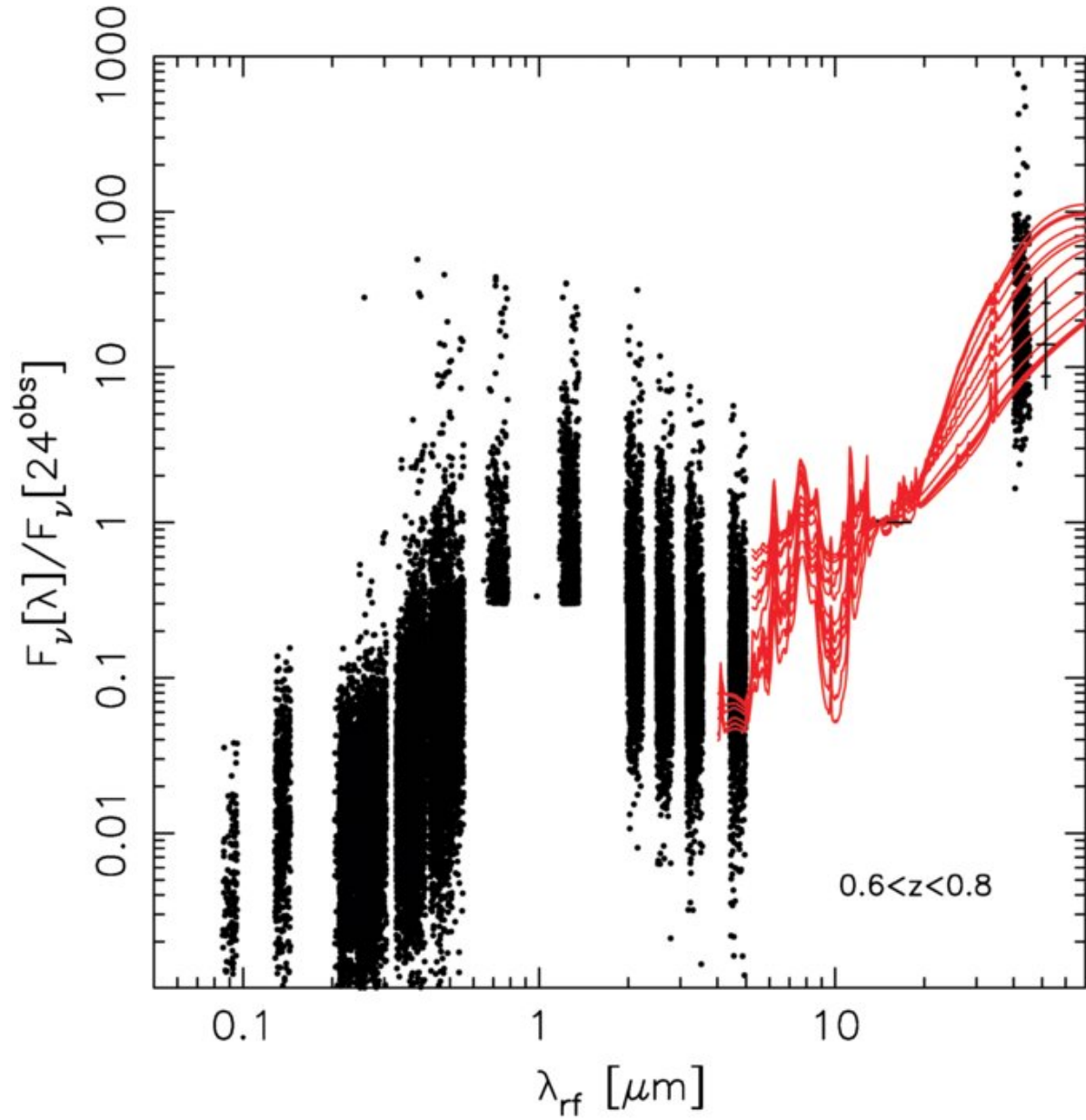
Figure 18. from Determining Star Formation Rates for Infrared Galaxies RIEKE ET AL. 2009 ApJ 692 556 doi:10.1088/0004-637X/692/1/556 https://dx.doi.org/10.1088/0004-637X/692/1/556 © 2009. The American Astronomical Society. All rights reserved.
