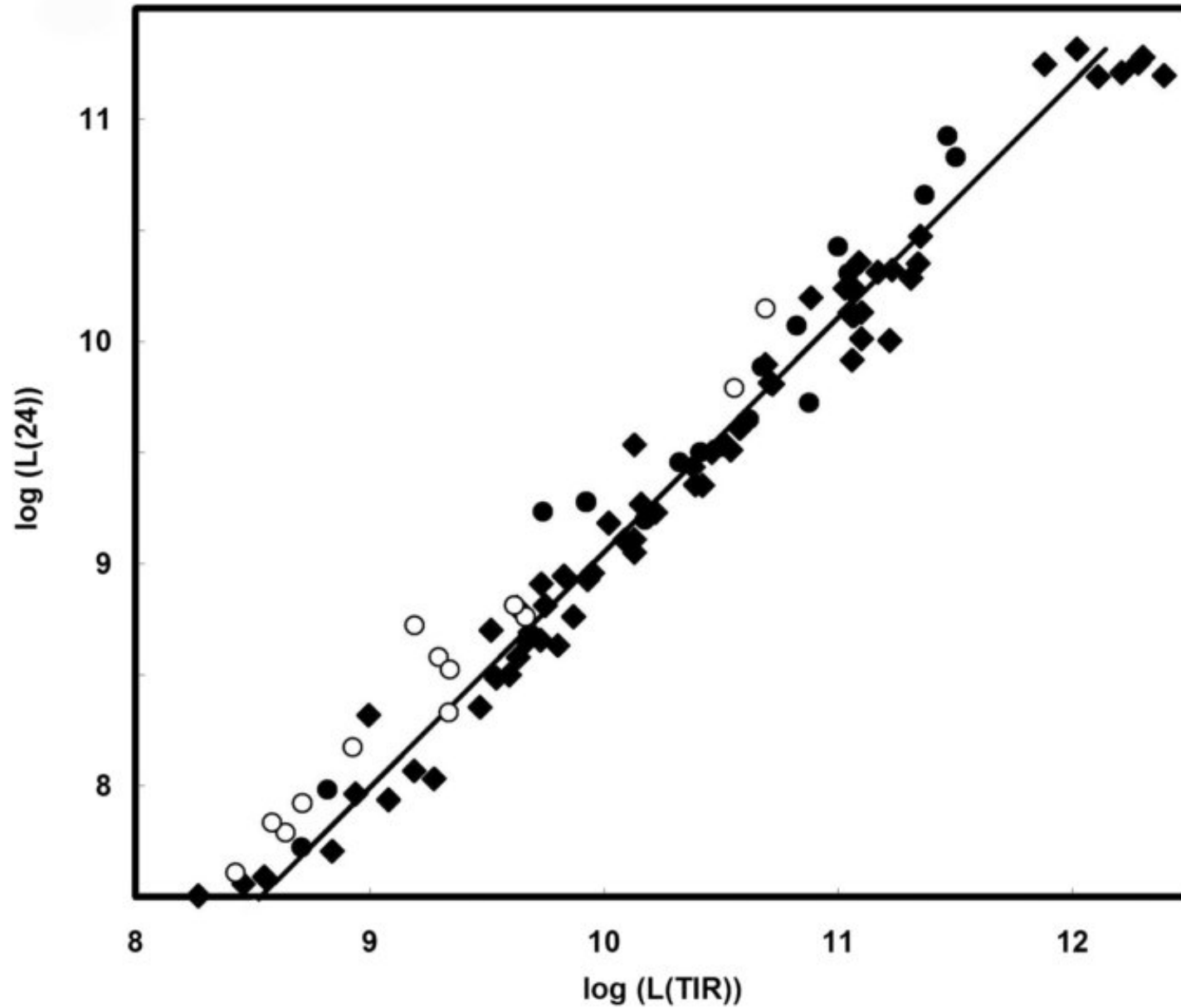
Figure 15. from Determining Star Formation Rates for Infrared Galaxies RIEKE ET AL. 2009 ApJ 692 556 doi:10.1088/0004-637X/692/1/556 https://dx.doi.org/10.1088/0004-637X/692/1/556 © 2009. The American Astronomical Society. All rights reserved.
