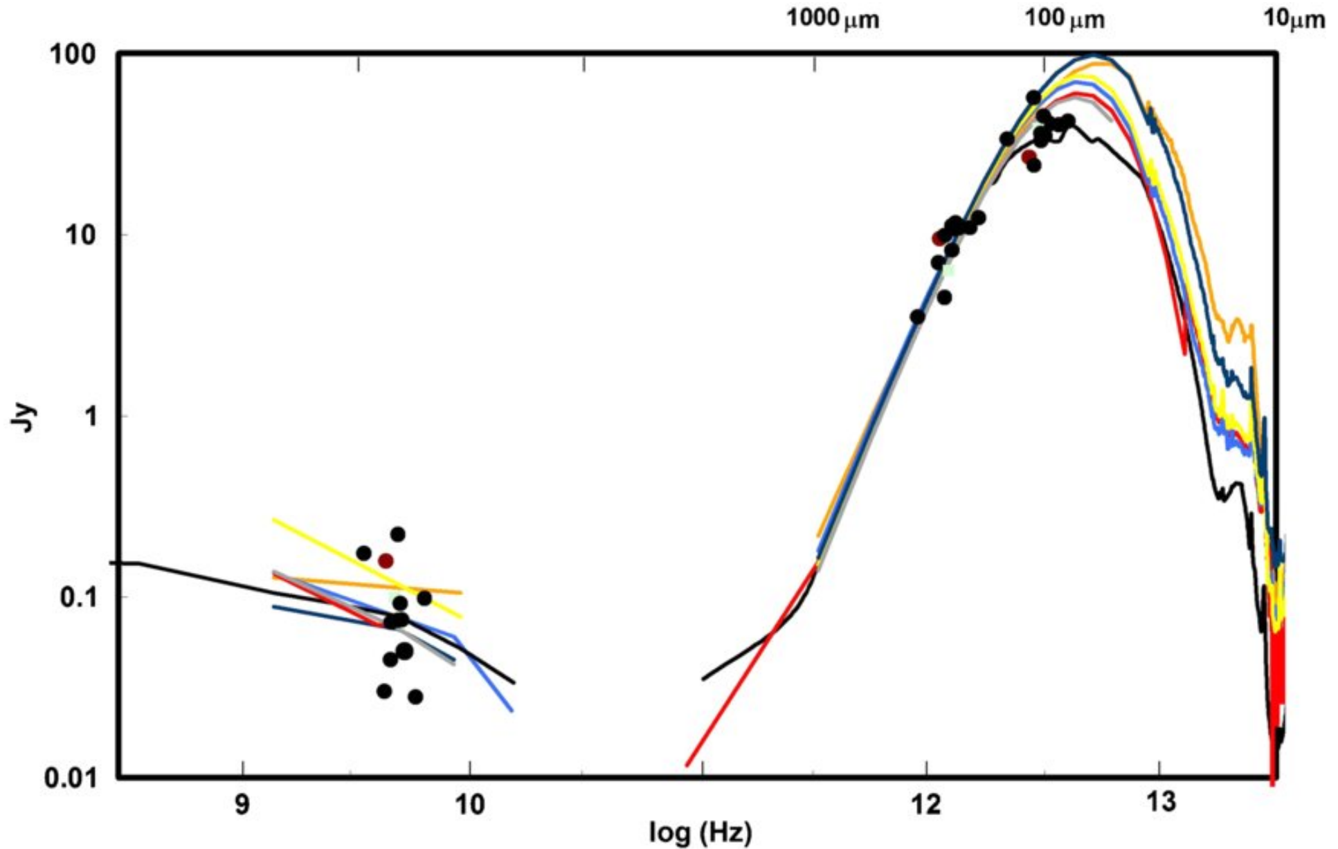
Figure 12. from Determining Star Formation Rates for Infrared Galaxies RIEKE ET AL. 2009 ApJ 692 556 doi:10.1088/0004-637X/692/1/556 https://dx.doi.org/10.1088/0004-637X/692/1/556 © 2009. The American Astronomical Society. All rights reserved.
