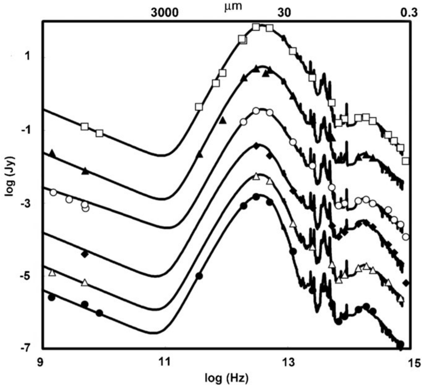
Figure 1. from Determining Star Formation Rates for Infrared Galaxies RIEKE ET AL. 2009 ApJ 692 556 doi:10.1088/0004-637X/692/1/556 https://dx.doi.org/10.1088/0004-637X/692/1/556 © 2009. The American Astronomical Society. All rights reserved.
