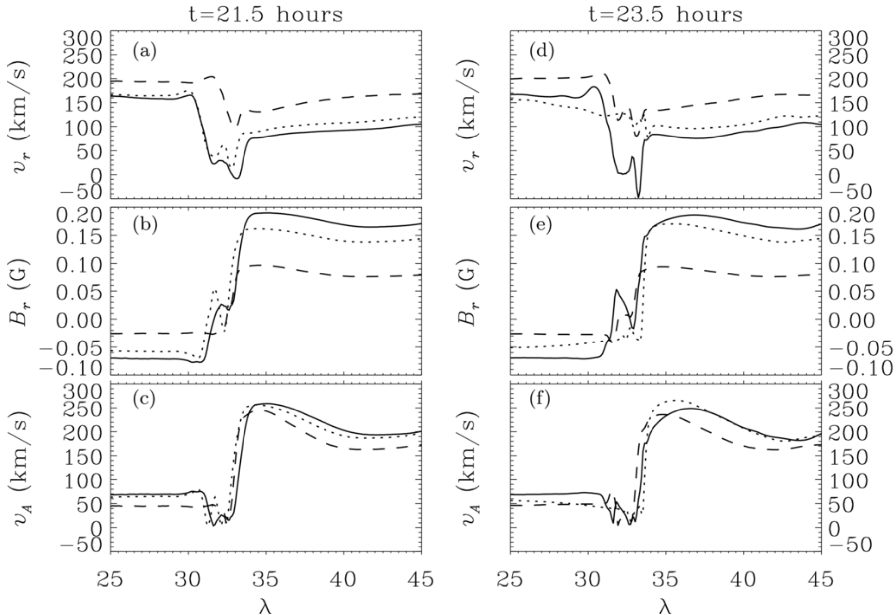
Figure 3. from Intrinsic Instability of Coronal Streamers CHEN ET AL. 2009 ApJ 691 1936 doi:10.1088/0004-637X/691/2/1936 https://dx.doi.org/10.1088/0004-637X/691/2/1936 © 2009. The American Astronomical Society. All rights reserved.
