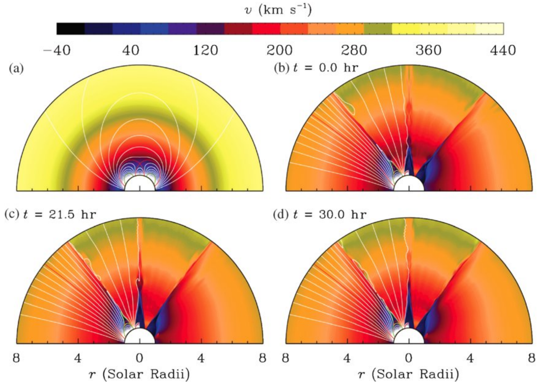
Figure 1. from Intrinsic Instability of Coronal Streamers CHEN ET AL. 2009 ApJ 691 1936 doi:10.1088/0004-637X/691/2/1936 https://dx.doi.org/10.1088/0004-637X/691/2/1936 © 2009. The American Astronomical Society. All rights reserved.
