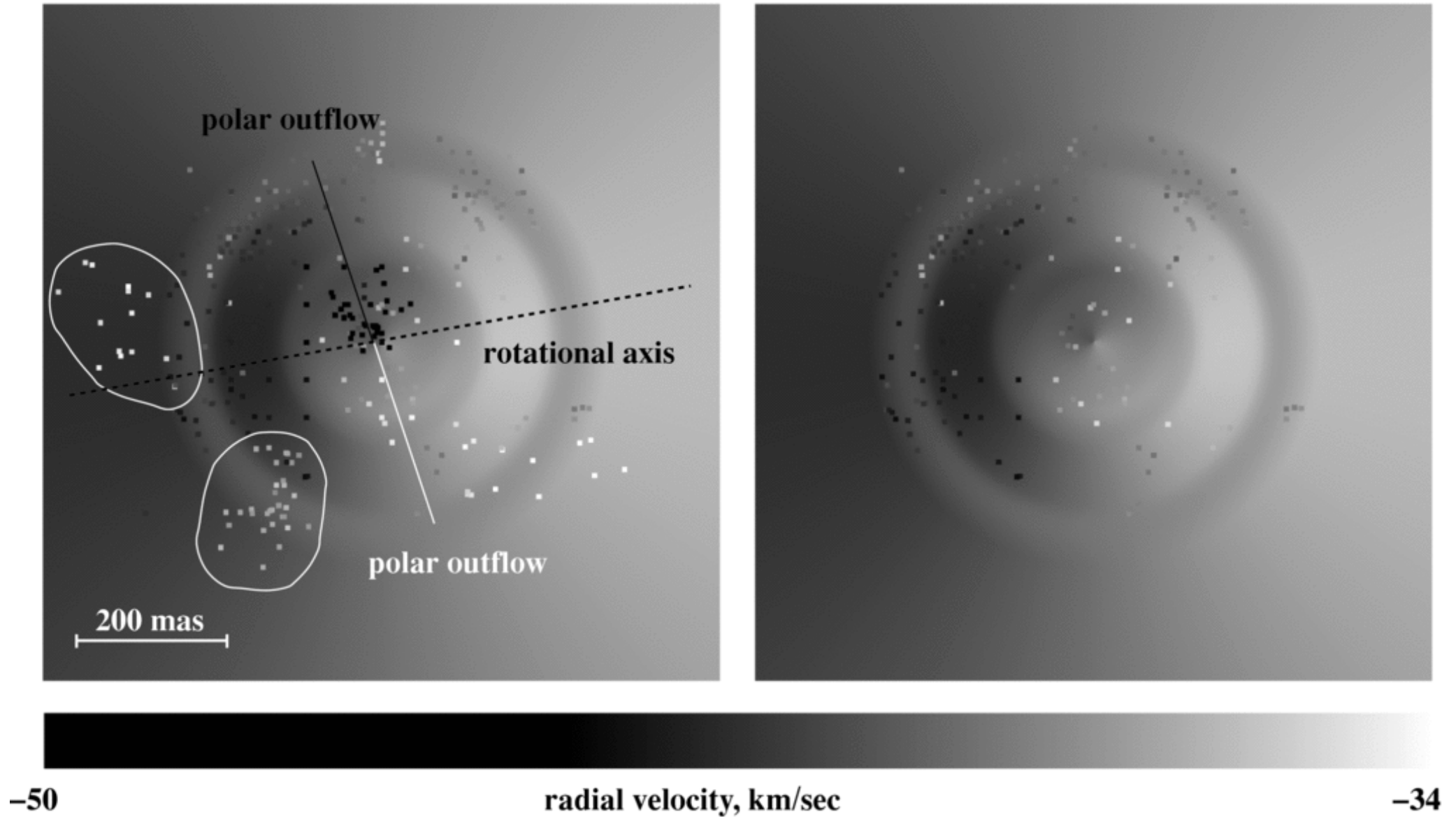
Figure 8. from The Structure and Kinematics of the Envelope Around U Ori from Iota Observations PLUZHNIK ET AL. 2009 ApJ 700 114 doi:10.1088/0004-637X/700/1/114 https://dx.doi.org/10.1088/0004-637X/700/1/114 © 2009. The American Astronomical Society. All rights reserved.
