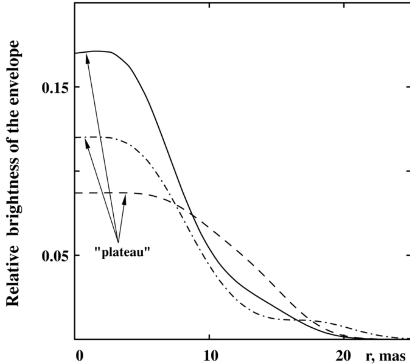
Figure 4. from The Structure and Kinematics of the Envelope Around U Ori from Iota Observations PLUZHNIK ET AL. 2009 ApJ 700 114 doi:10.1088/0004-637X/700/1/114 https://dx.doi.org/10.1088/0004-637X/700/1/114 © 2009. The American Astronomical Society. All rights reserved.
