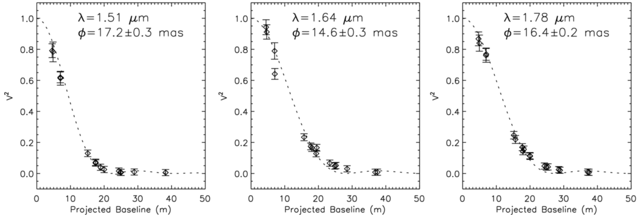
Figure 2. from The Structure and Kinematics of the Envelope Around U Ori from Iota Observations PLUZHNIK ET AL. 2009 ApJ 700 114 doi:10.1088/0004-637X/700/1/114 https://dx.doi.org/10.1088/0004-637X/700/1/114 © 2009. The American Astronomical Society. All rights reserved.
