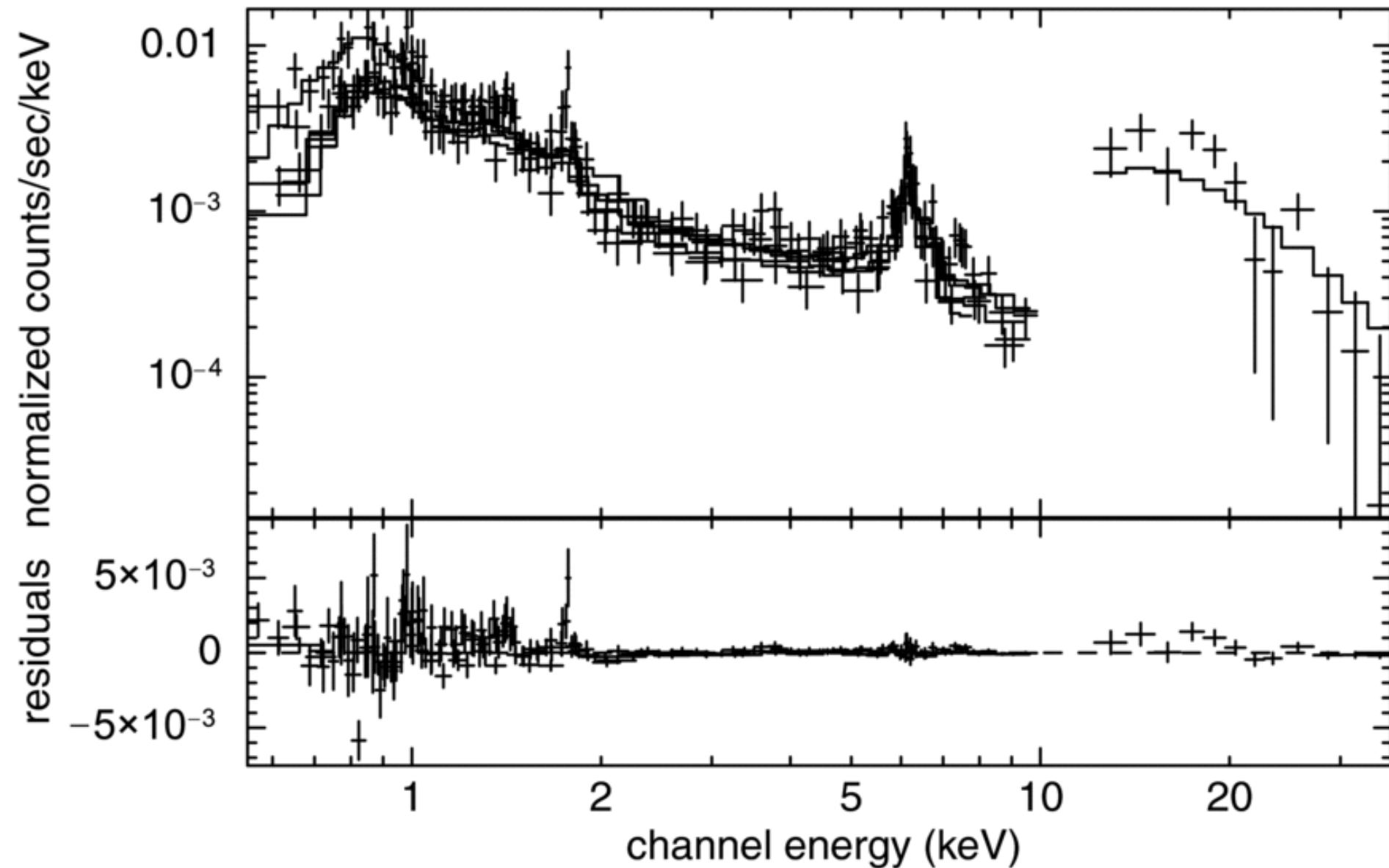
Figure 4. from Suzaku Observations of Local Ultraluminous Infrared Galaxies TENG ET AL. 2009 ApJ 691 261 doi:10.1088/0004-637X/691/1/261 https://dx.doi.org/10.1088/0004-637X/691/1/261 © 2009. The American Astronomical Society. All rights reserved.
