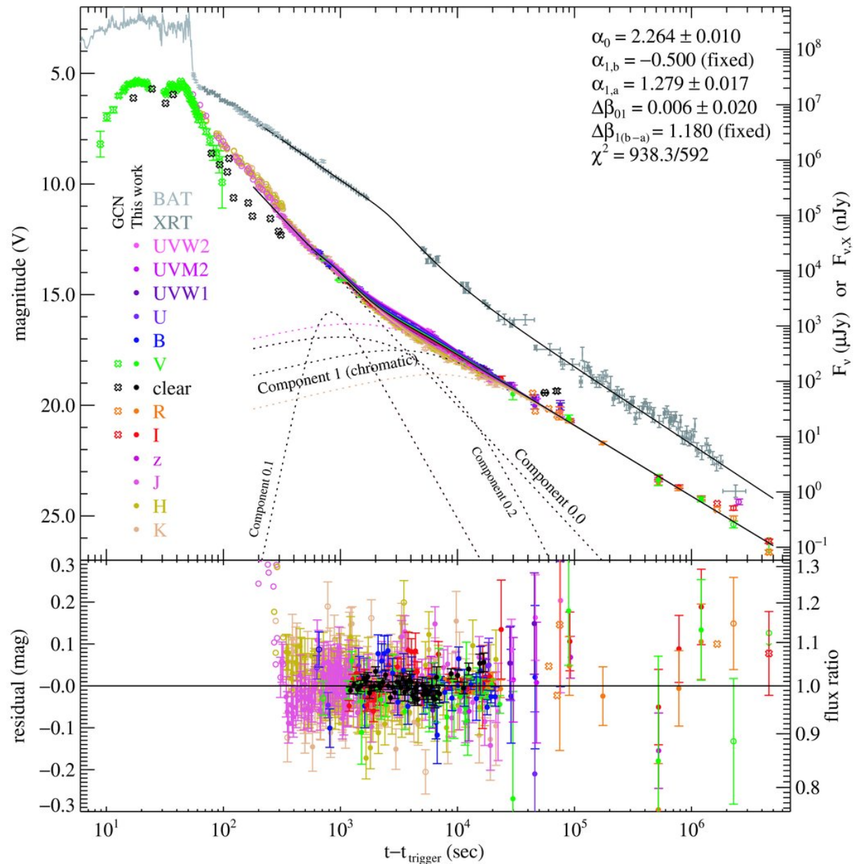
Figure 1. from Observations of the Naked-Eye GRB 080319B: Implications of Nature's Brightest Explosion BLOOM ET AL. 2009 ApJ 691 723 doi:10.1088/0004-637X/691/1/723 https://dx.doi.org/10.1088/0004-637X/691/1/723 © 2009. The American Astronomical Society. All rights reserved.
