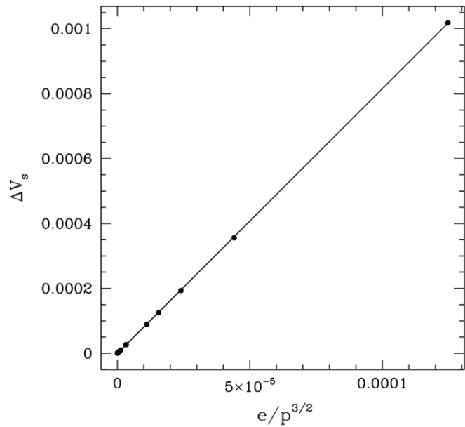
Figure 4. from Frame Dragging and the Kinematics of Galactic-Center Stars KANNAN & SAHA 2009 ApJ 690 1553 doi:10.1088/0004-637X/690/2/1553 https://dx.doi.org/10.1088/0004-637X/690/2/1553 © 2009. The American Astronomical Society. All rights reserved.
