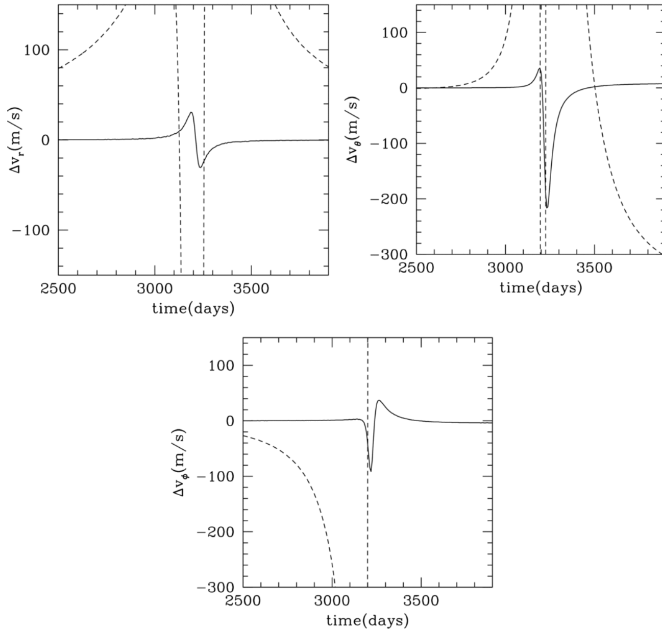
Figure 3. from Frame Dragging and the Kinematics of Galactic-Center Stars KANNAN & SAHA 2009 ApJ 690 1553 doi:10.1088/0004-637X/690/2/1553 https://dx.doi.org/10.1088/0004-637X/690/2/1553 © 2009. The American Astronomical Society. All rights reserved.
