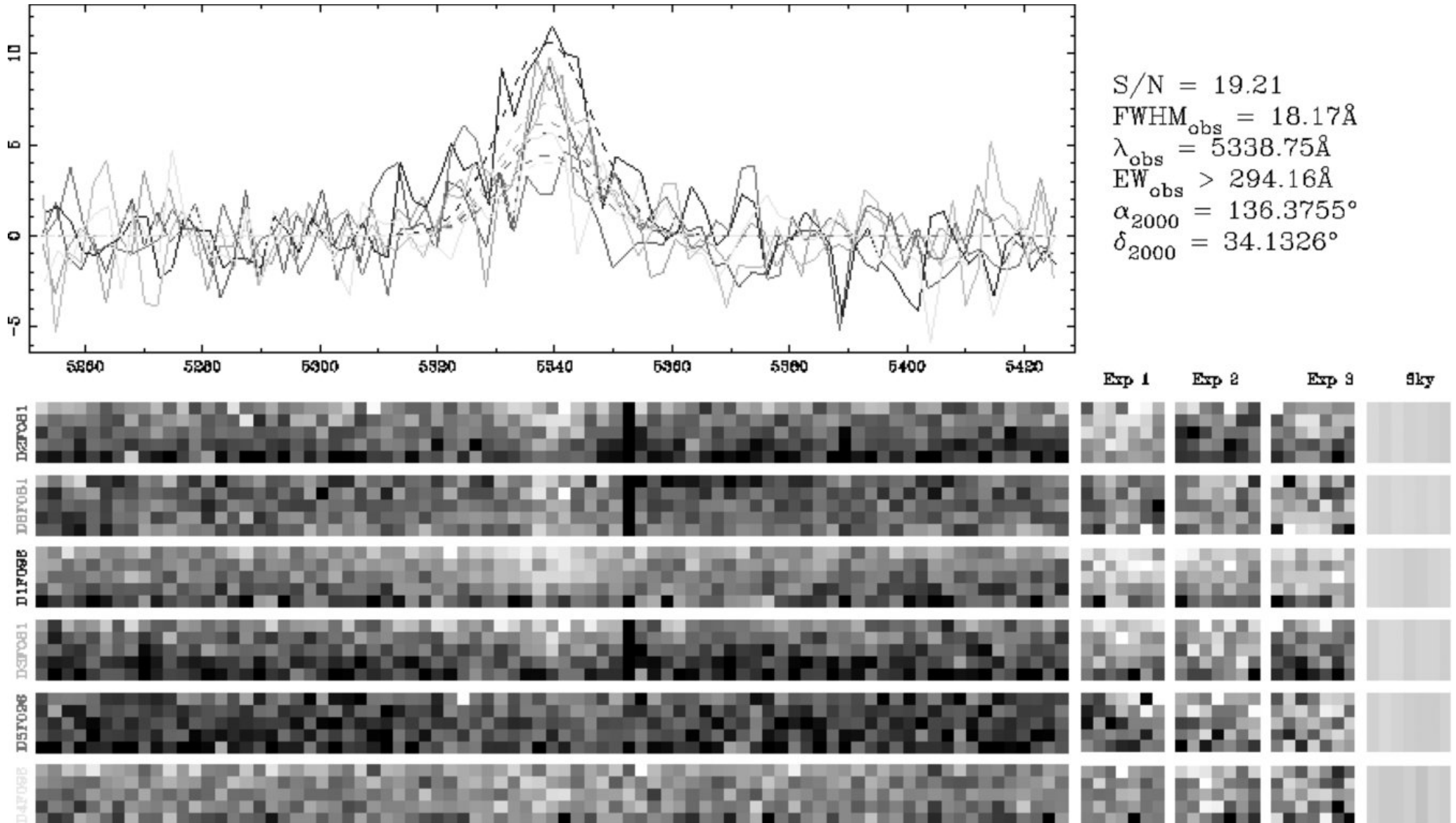
Figure 4. from B2 0902+34: A Collapsing Protogiant Elliptical Galaxy at z = 3.4 ADAMS, HILL, & MACQUEEN 2009 ApJ 694 314 doi:10.1088/0004-637X/694/1/314 https://dx.doi.org/10.1088/0004-637X/694/1/314 © 2009. The American Astronomical Society. All rights reserved.
