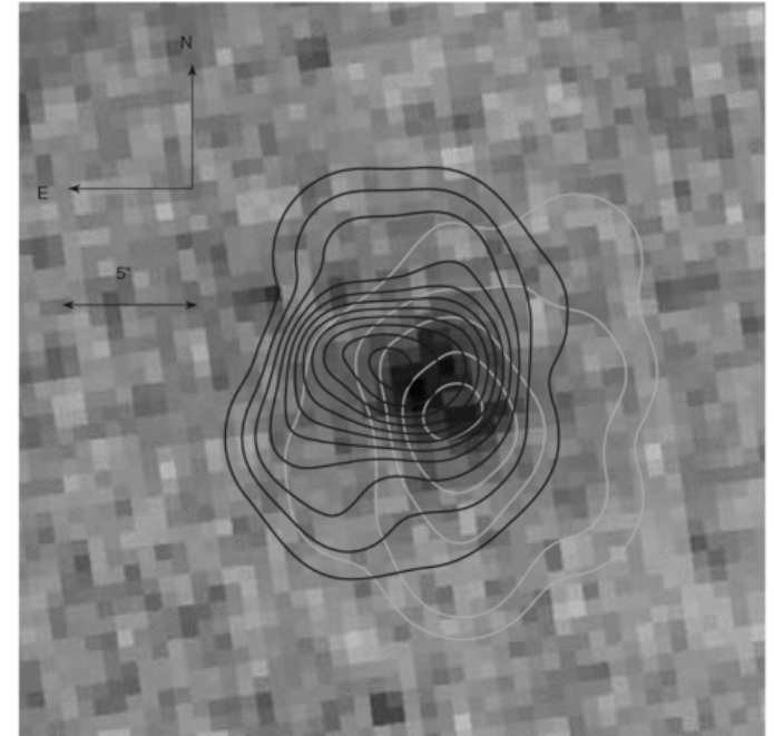
(c) Simulated, Origin Cone Decomposition
