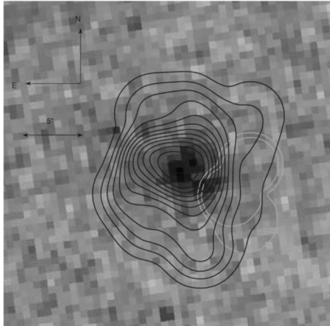
(b) Simulated, Spectral Decomposition
