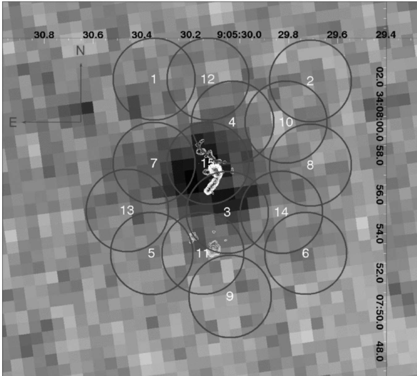
Figure 1. from B2 0902+34: A Collapsing Protogiant Elliptical Galaxy at z = 3.4 ADAMS, HILL, & MACQUEEN 2009 ApJ 694 314 doi:10.1088/0004-637X/694/1/314 https://dx.doi.org/10.1088/0004-637X/694/1/314 © 2009. The American Astronomical Society. All rights reserved.
