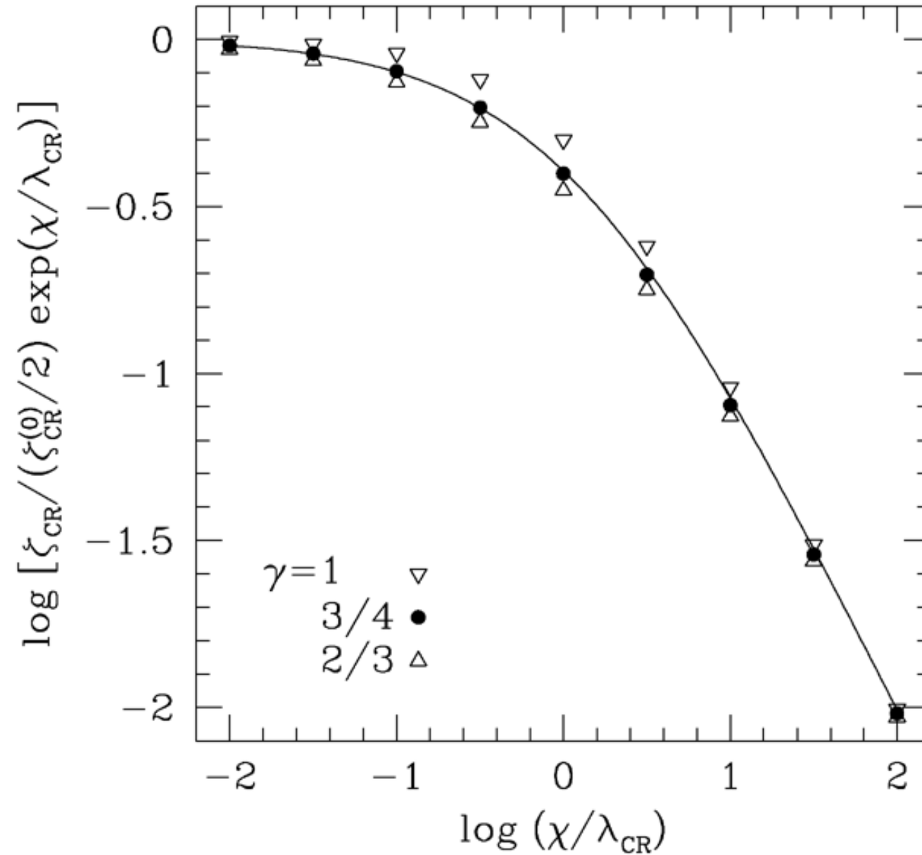
Figure 4. from Effects of Radionuclides on the Ionization State of Protoplanetary Disks and Dense Cloud Cores UMEBAYASHI & NAKANO 2009 ApJ 690 69 doi:10.1088/0004-637X/690/1/69 https://dx.doi.org/10.1088/0004-637X/690/1/69 © 2009. The American Astronomical Society. All rights reserved.
