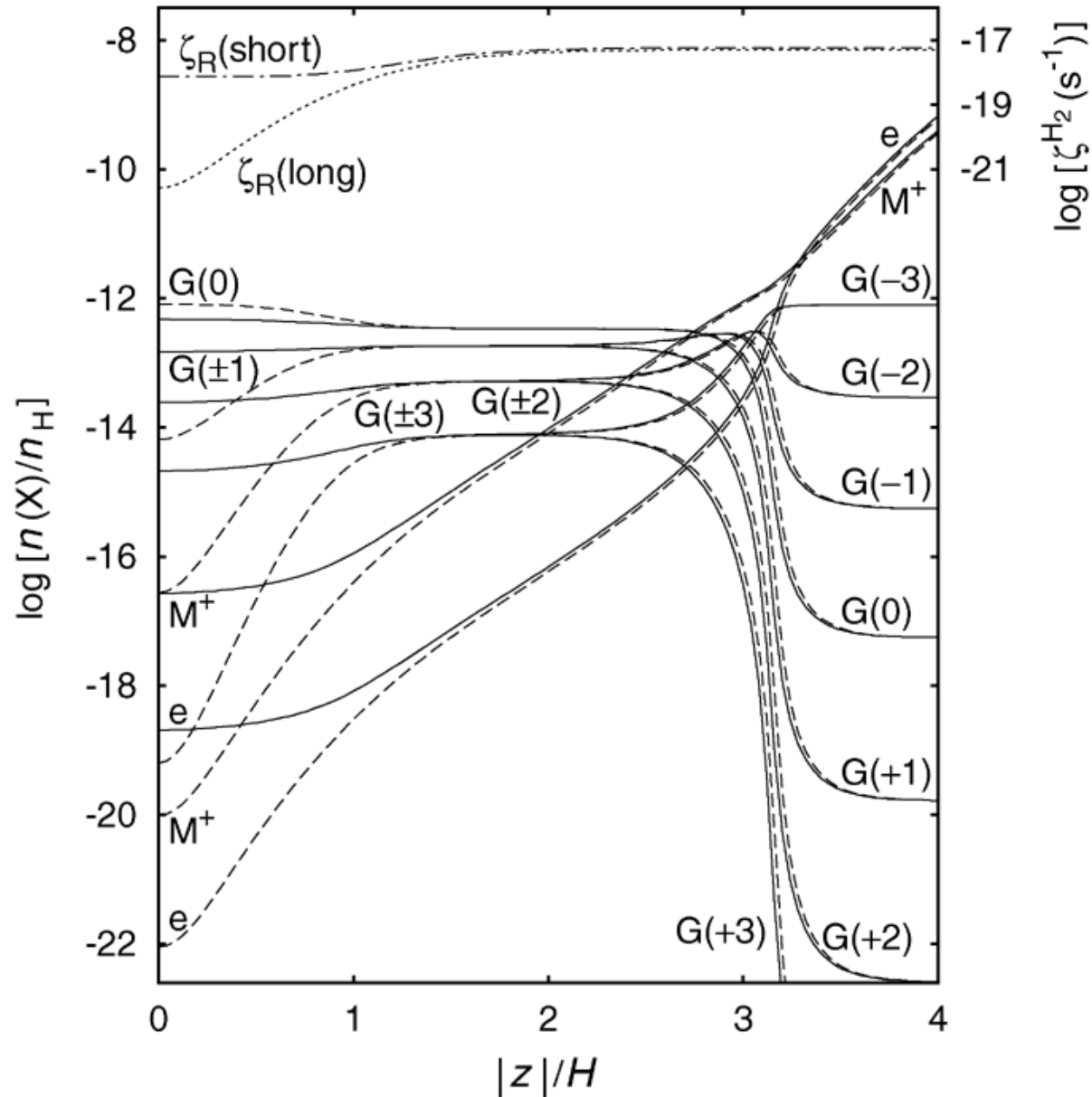
Figure 3. from Effects of Radionuclides on the Ionization State of Protoplanetary Disks and Dense Cloud Cores UMEBAYASHI & NAKANO 2009 ApJ 690 69 doi:10.1088/0004-637X/690/1/69 https://dx.doi.org/10.1088/0004-637X/690/1/69 © 2009. The American Astronomical Society. All rights reserved.
