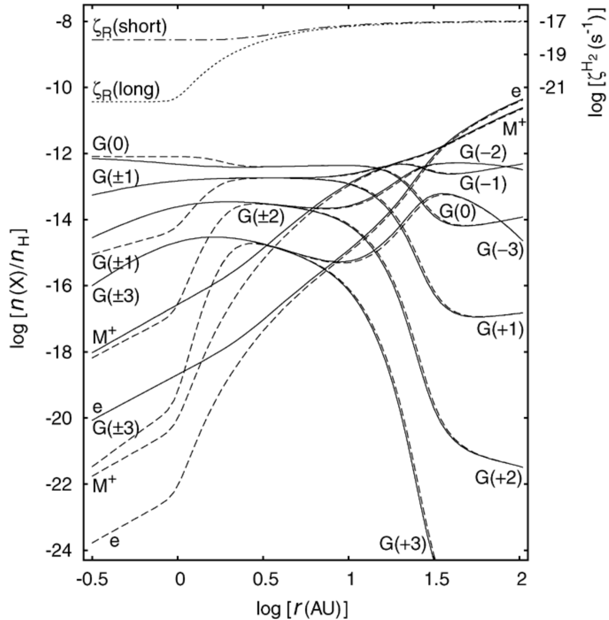
Figure 2. from Effects of Radionuclides on the Ionization State of Protoplanetary Disks and Dense Cloud Cores UMEBAYASHI & NAKANO 2009 ApJ 690 69 doi:10.1088/0004-637X/690/1/69 https://dx.doi.org/10.1088/0004-637X/690/1/69 © 2009. The American Astronomical Society. All rights reserved.
