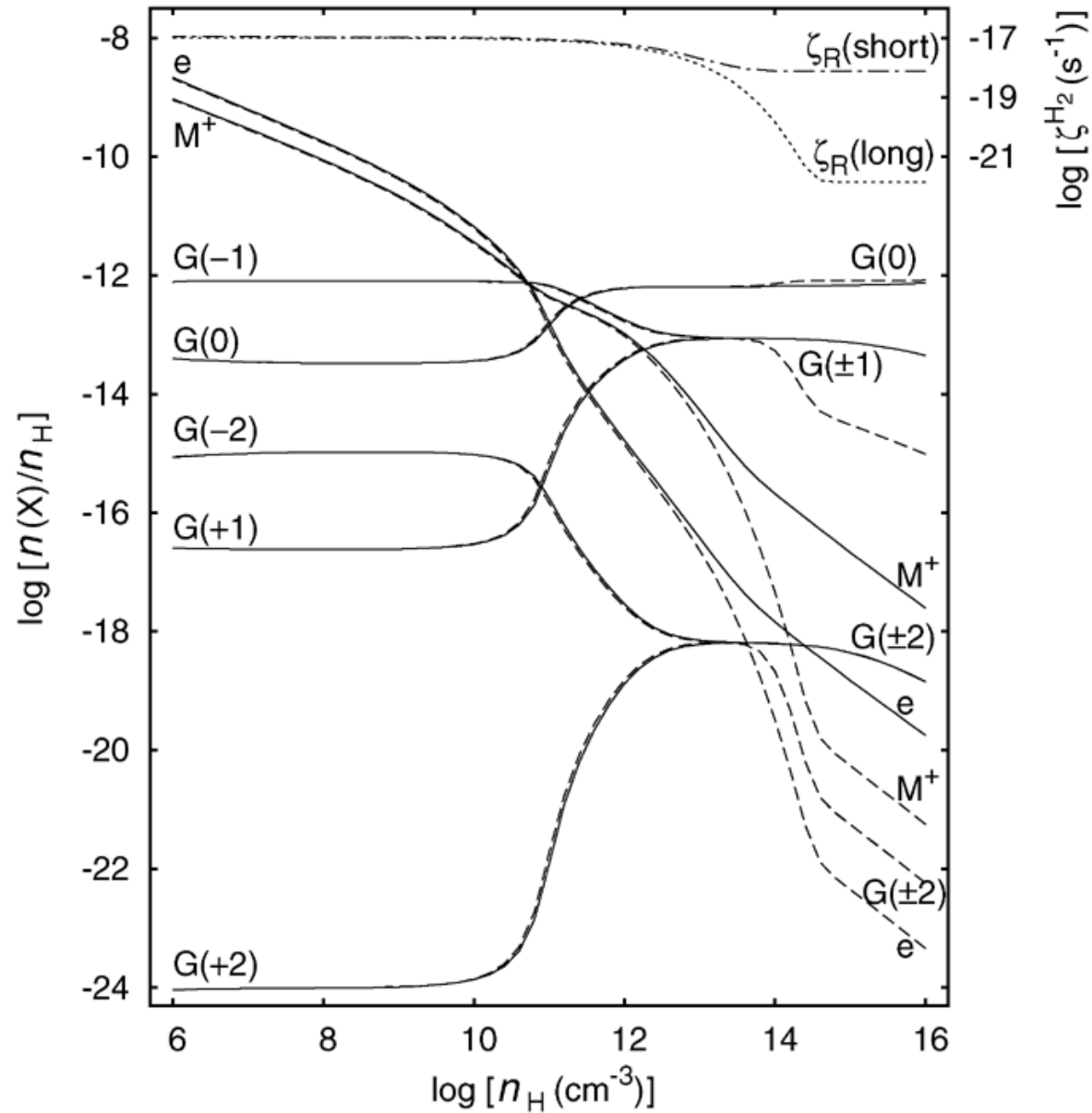
Figure 1. from Effects of Radionuclides on the Ionization State of Protoplanetary Disks and Dense Cloud Cores UMEBAYASHI & NAKANO 2009 ApJ 690 69 doi:10.1088/0004-637X/690/1/69 https://dx.doi.org/10.1088/0004-637X/690/1/69 © 2009. The American Astronomical Society. All rights reserved.
