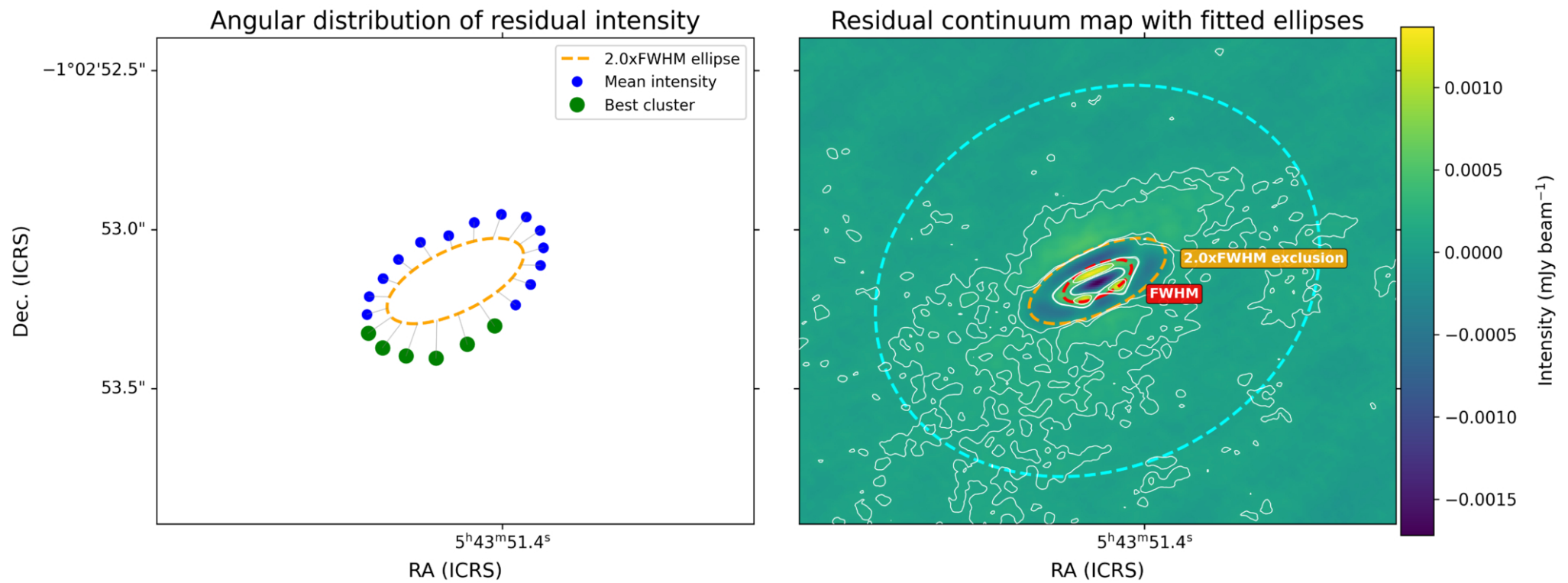
Figure D2. from Adele L. Plunkett et al 2026 Astron. J. 172 doi:10.3847/1538-3881/aeacc2 https://dx.doi.org/10.3847/1538-3881/aeacc2 © 2026. The Author(s). Published by the American Astronomical Society.
